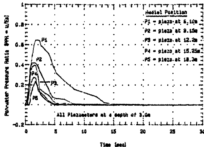
Figure 6.9 Residual porewater pressure expressed as the dimensionless porewater pressure ratio, (PPR = u/\sigma') , vs. time after detonation number six, (9.1030 kg).
