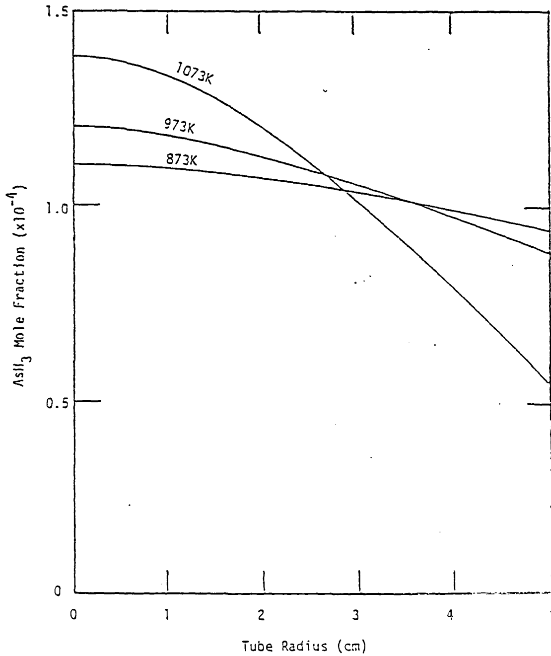
Figure A-16 \text{AsH}_3 Radial Composition Profile at 99% Decomposition
