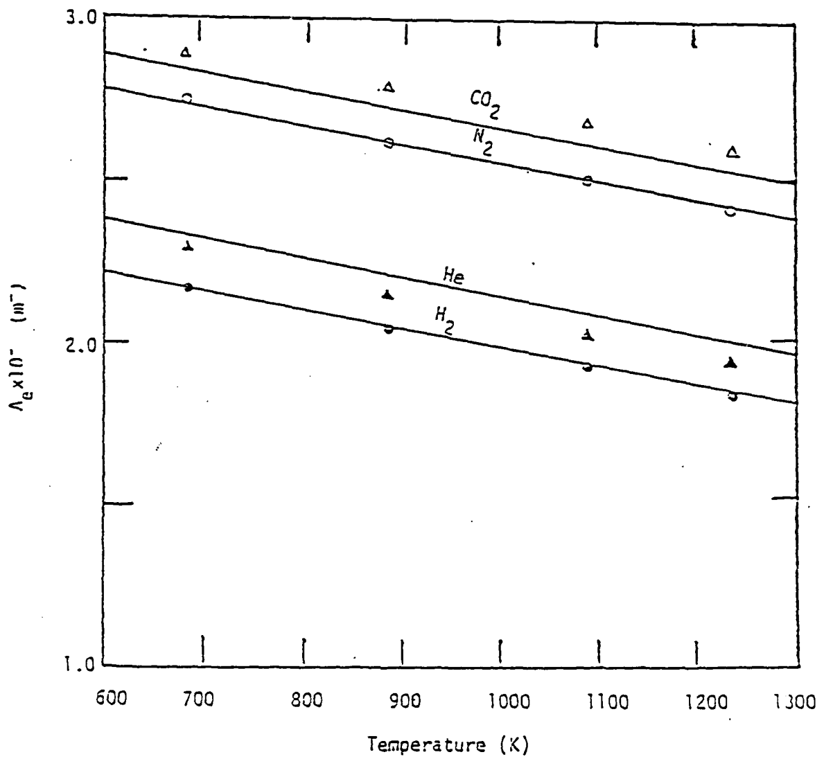
Figure A-4 Orifice Calibration Results (• \text{H}_2 , \blacktriangle \text{He} , \circ \text{H}_2 , \triangle \text{CO}_2 )
