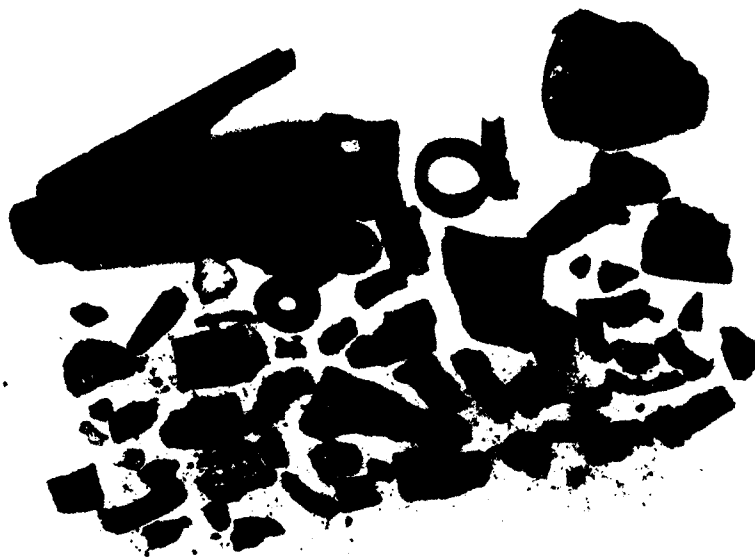
FIG. 1 CPMI body fractured by 10 g Tetryl Charge
