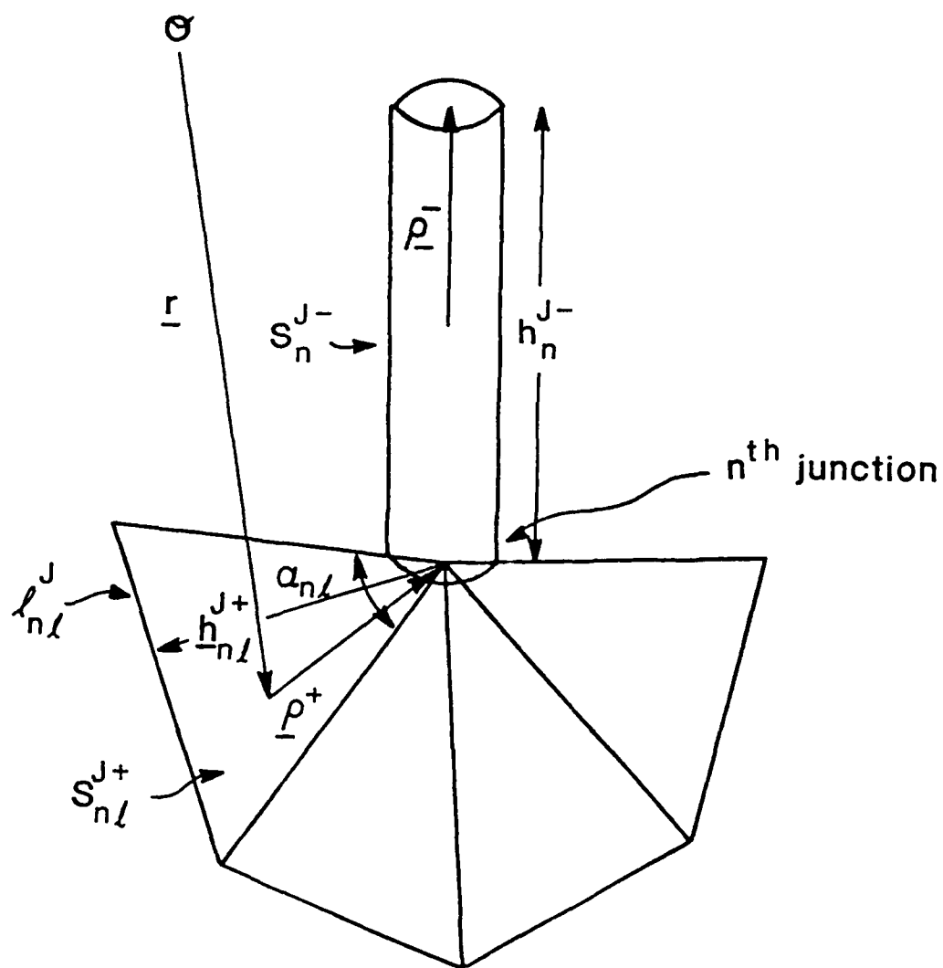
Figure 3.4: Geometrical parameters associated with the n th wire-to-surface junction.
