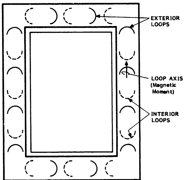
B. Loops Around Door
