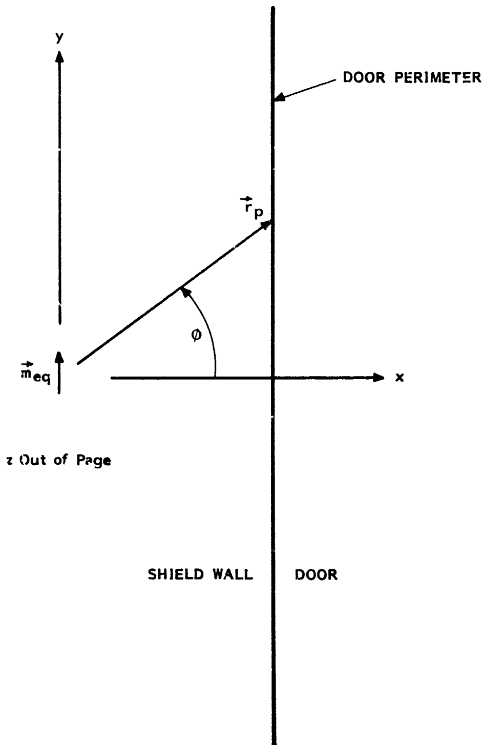
Figure 3.1. Location of Equivalent Magnetic Dipole with Respect to Door Perimeter
