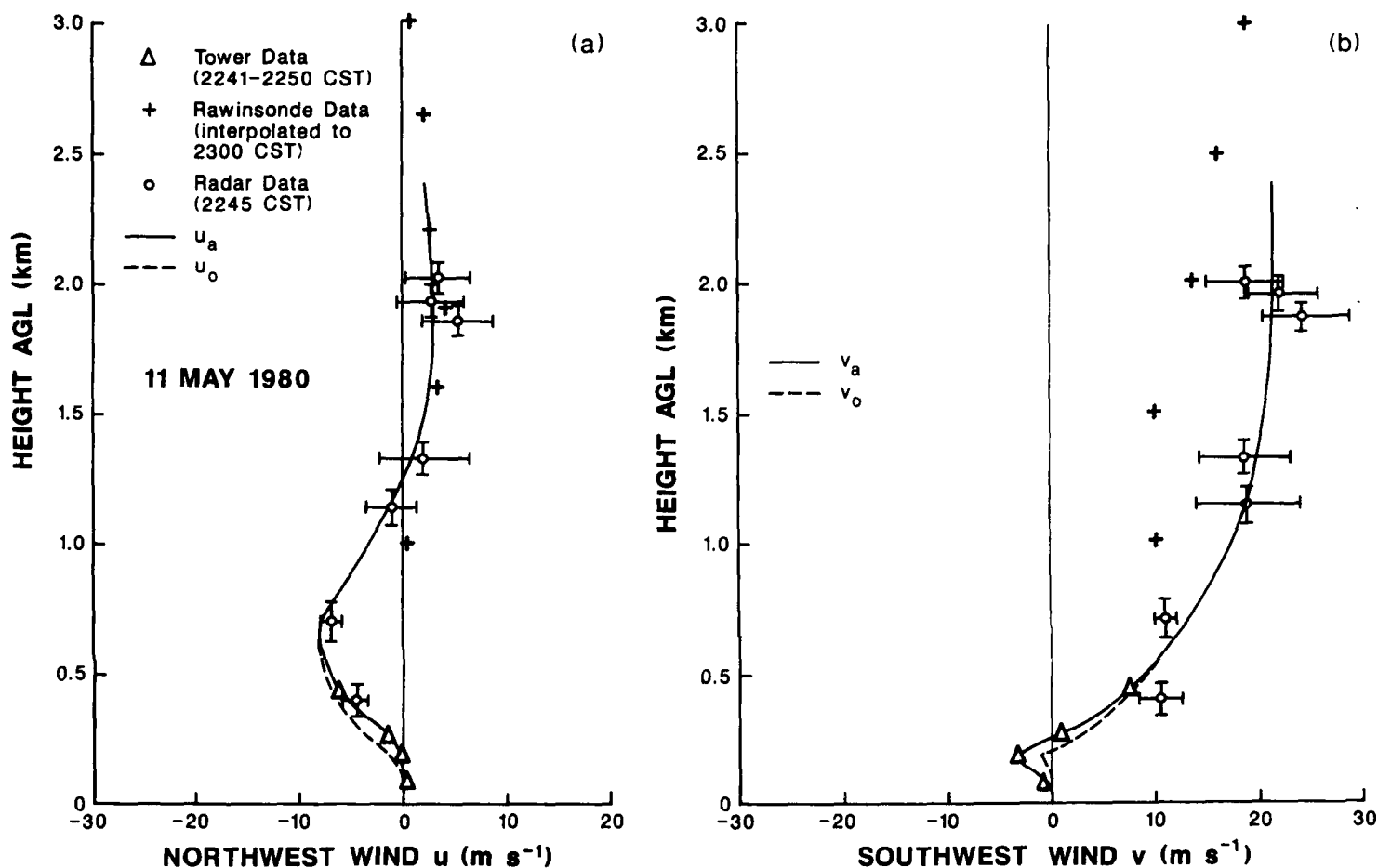
Figure 2a. The ambient wind component u_a, u_o in the direction of wave propagation. The \Delta are data, from tower anemometers, averaged over the indicated 10-minute period. The u_a curve is fitted to these data, whereas the u_o curve is obtained from fitting data averaged over a 2 min period just preceding wave arrival at the tower. Open circles are wind components derived from single Doppler data fields and + are winds interpolated from earlier and later rawinsonde data.
