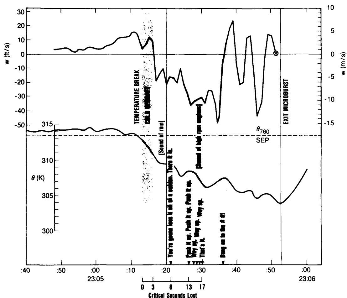
Figure 19b. A time series plot of vertical wind component (w) and static air temperature ( \theta ) from the Delta Flight 191 flight recorder together with comments from the flight crew that were recorded on the cockpit voice recorder (from Caracena et al., 1986).
