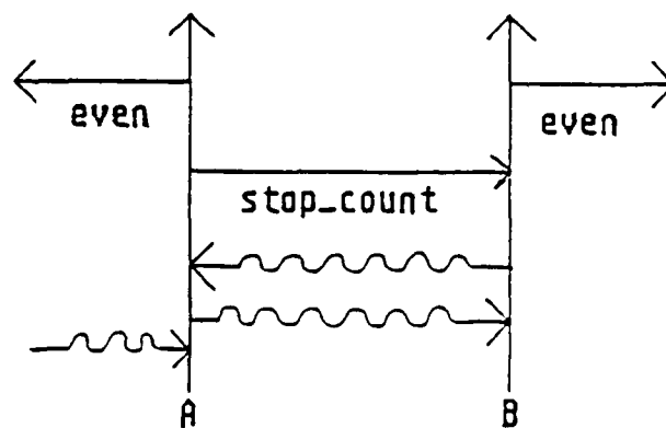
Figure 8.20: A "Fix Up" for B ; Not a Legal Trace for A
