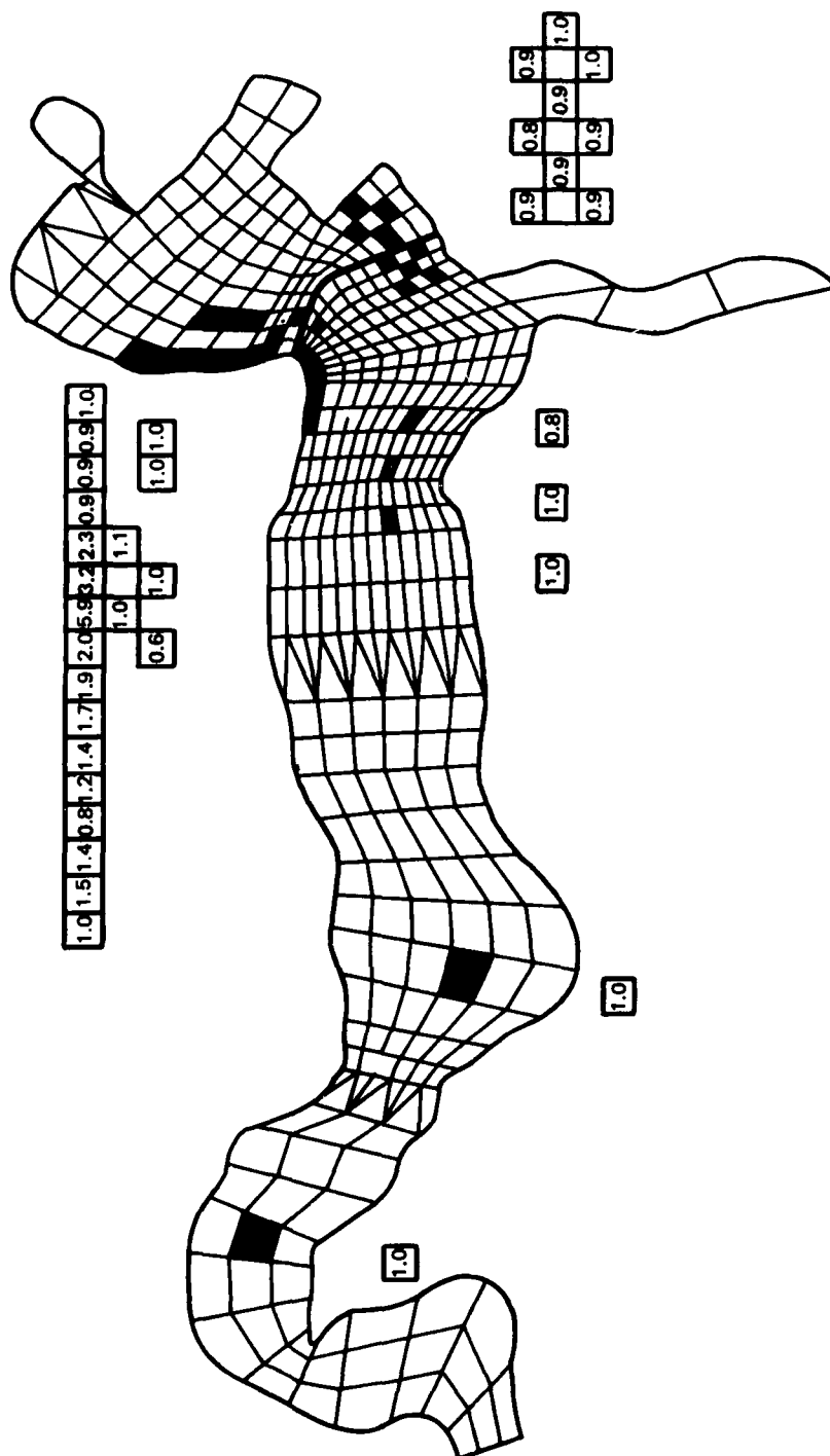
Figure 19. Yearly simulated shoaling indices
