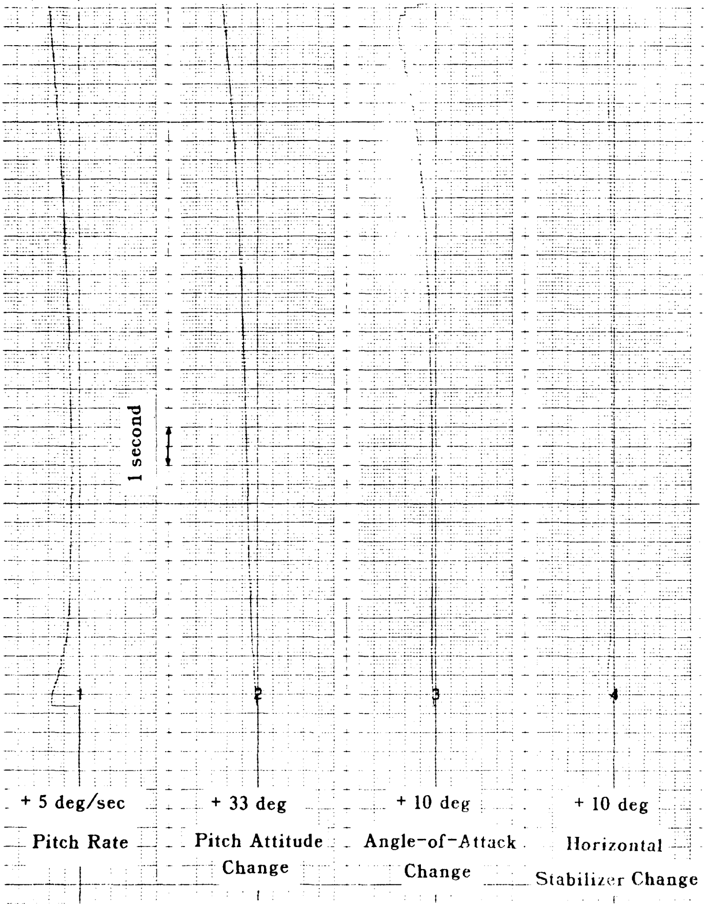
Figure 24. Stability Augmented Response without Angle-of-Attack
