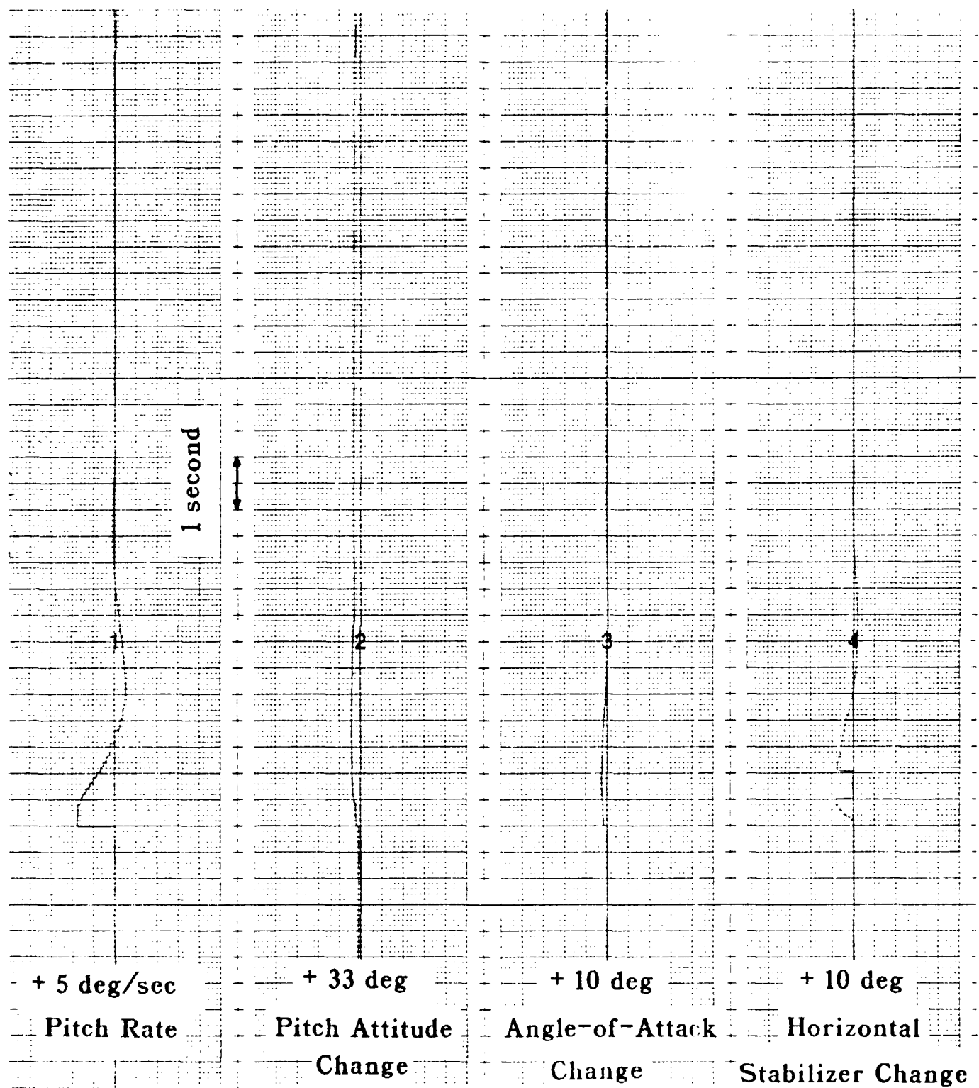
Figure 18. Augmented RSS Airplane Time History
