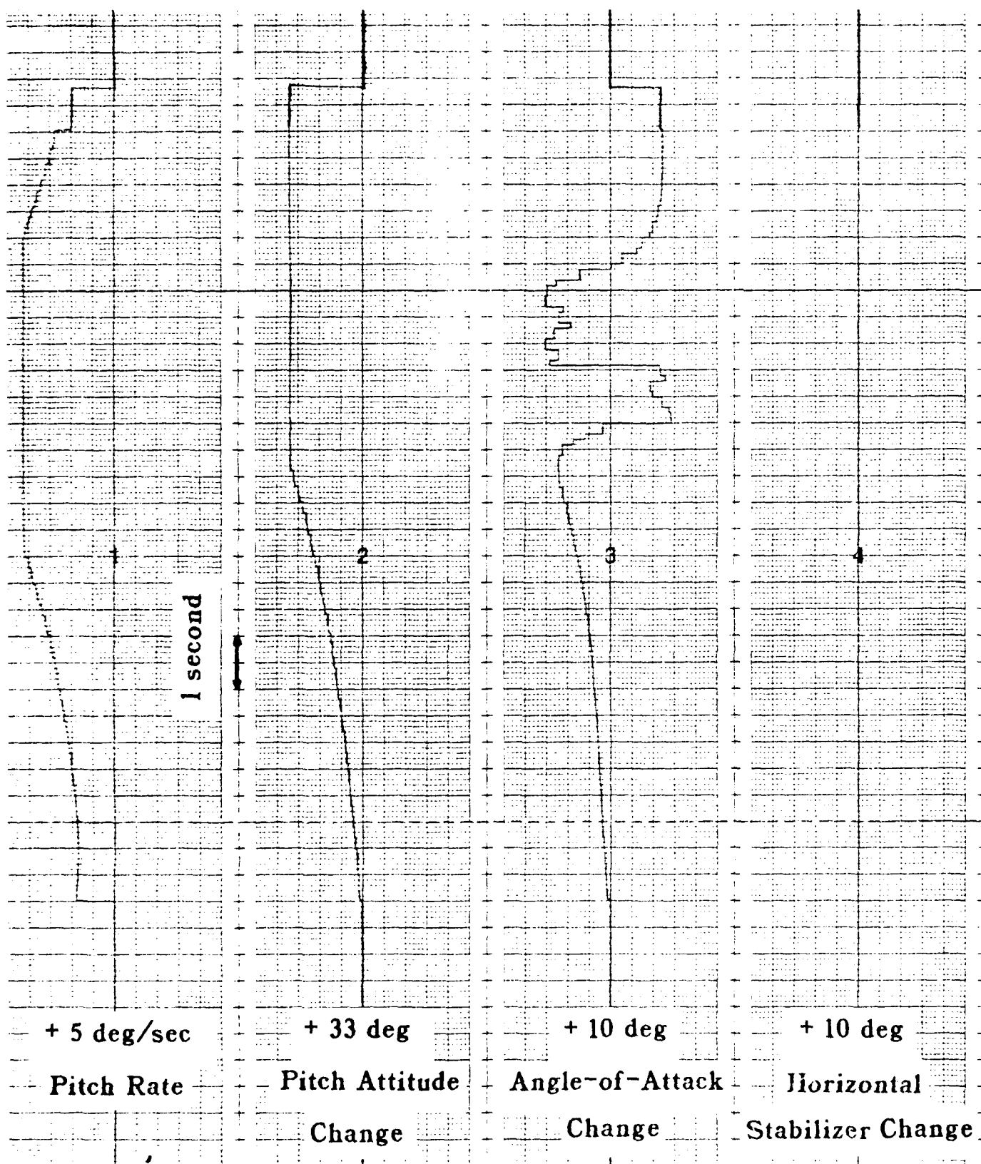
Figure 16. Free RSS Airplane Time History
