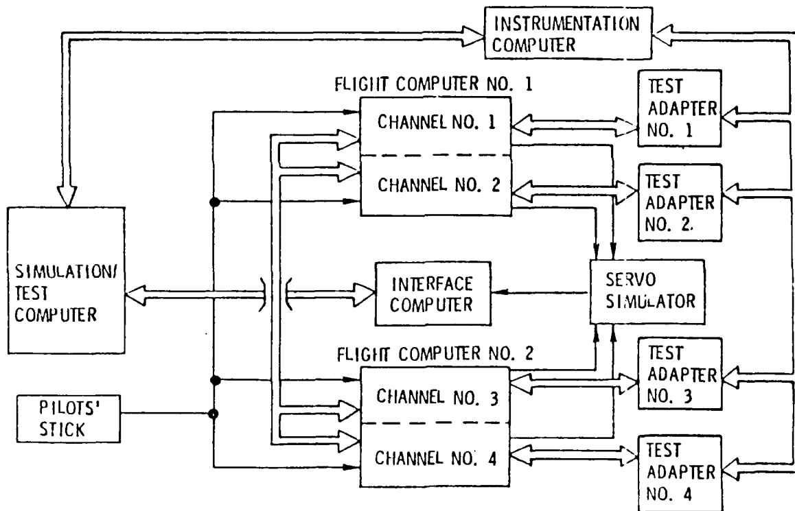
Figure E-2. RDFCS Facility Set-Up
