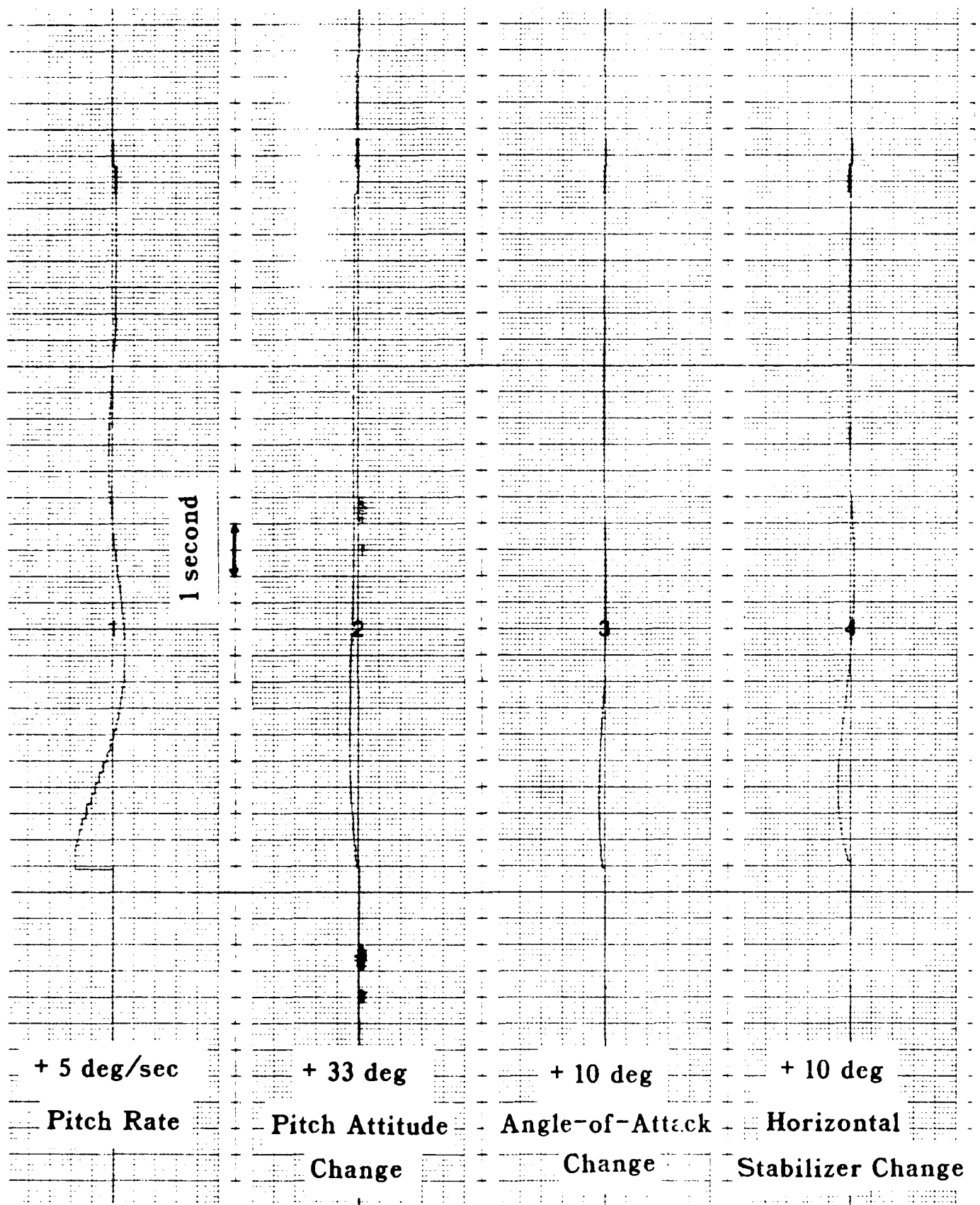
Figure 23. Stability Augmented Response without Pitch Rate
