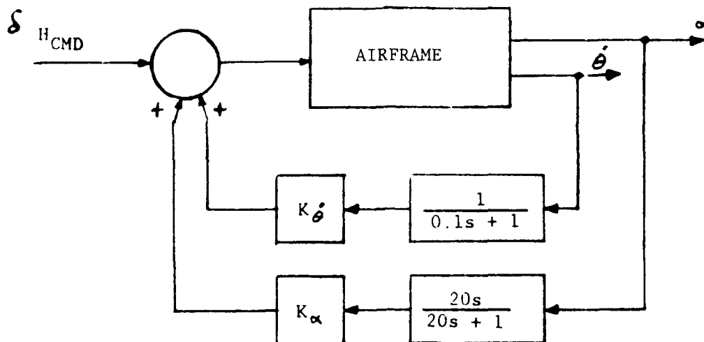
Figure 5. Augmented Fly-by-Wire Control Laws
