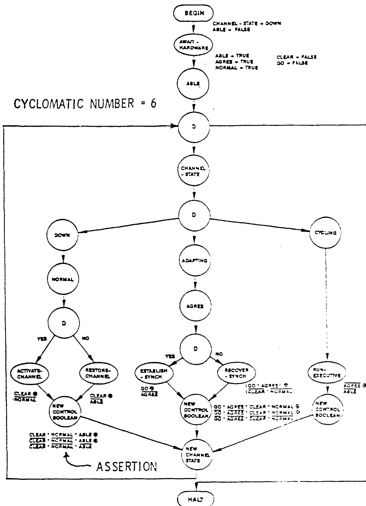
Figure 11. Top-Level Software Control Graph
