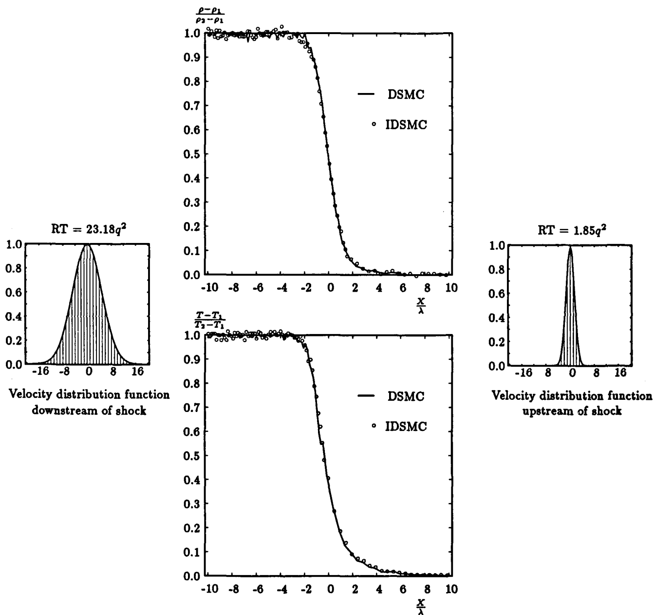
Figure 2.13. M_s = 6.11 Shock wave density and temperature profiles.
