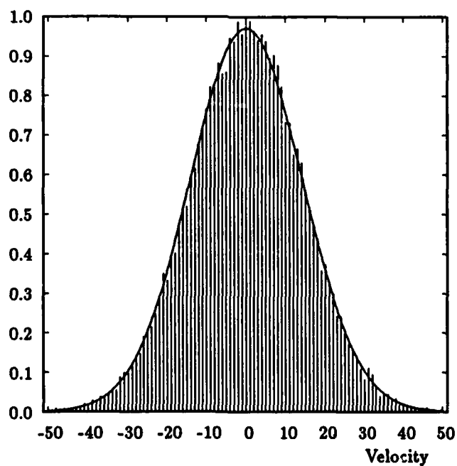
Figure 2.10b. Velocity component distribution function for RT = 201.3q^2 .
