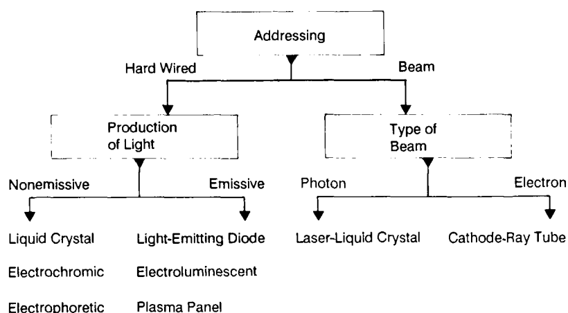
FIGURE 4.2 Examples of beam-addressed and matrix-addressed displays.
