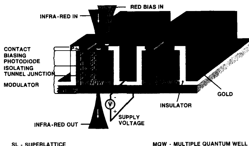
FIGURE 3.4 Three-dimensional schematic of an array of three-terminal optical logic devices. Each device consists of a photodiode, which absorbs the red bias input light, and a modulator (self-electrooptic effect device, or SEED), which has its infrared transmission controlled by the photodiode.
