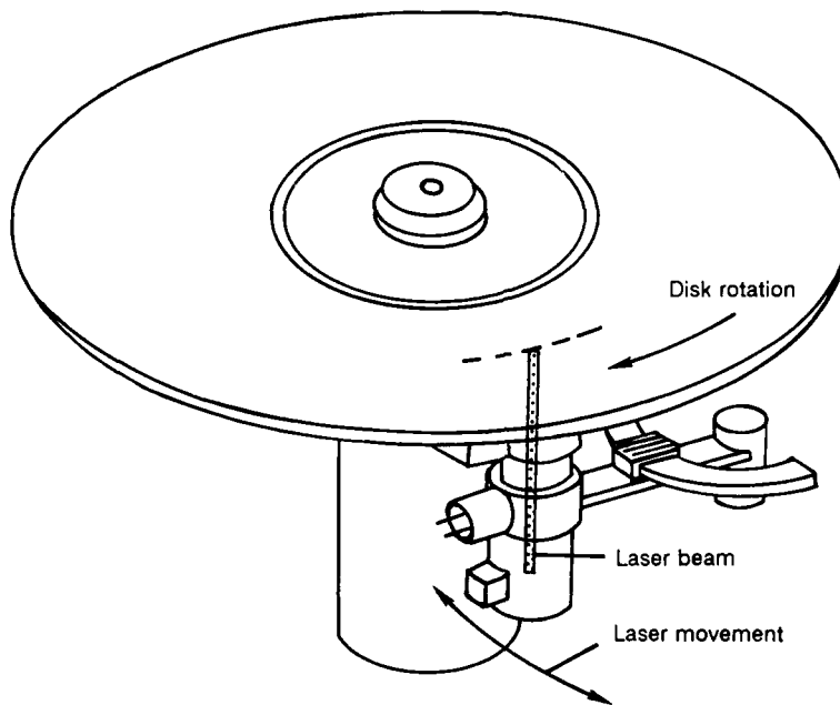
FIGURE 4.1 Diagram of optical storage system. The same laser may be used for both reading and writing.
