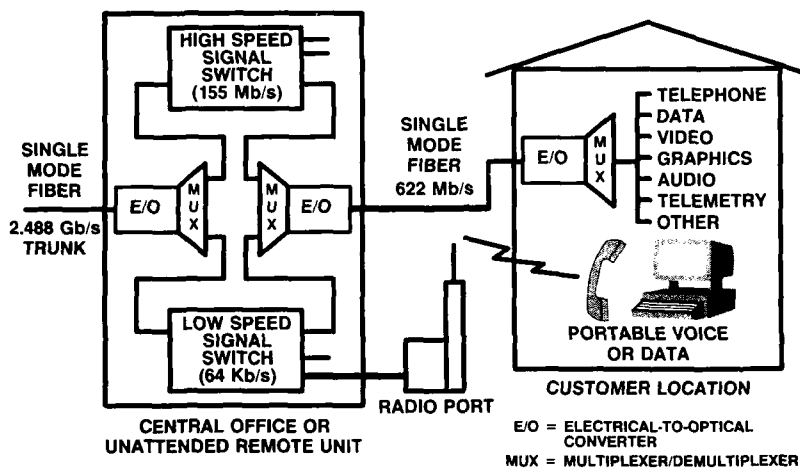
FIGURE 2.1 Setup for a typical office BISDN.
