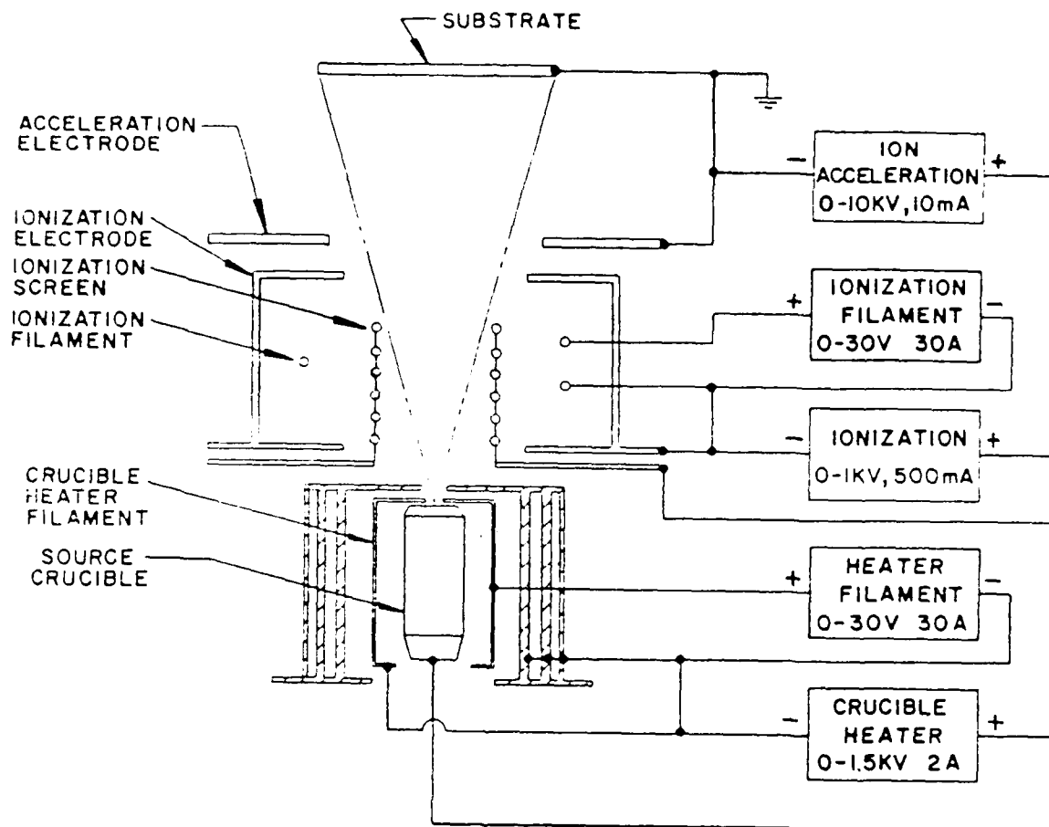
ION SOURCE ELECTRICAL SCHEMATIC
