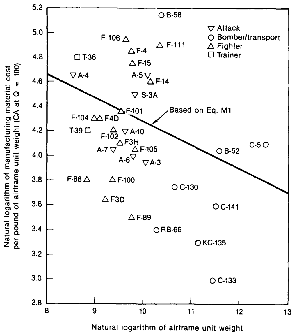
Fig. 6--Manufacturing material cost per pound as a function of airframe unit weight
