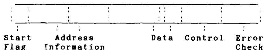
Fields present in a typical LAN packet
