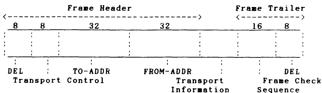
Packet structure of the IBM Token-Ring
