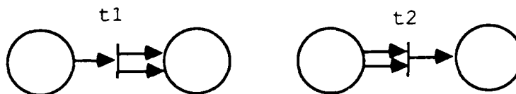
Figure 3-1. Basic Petri Net Structures
