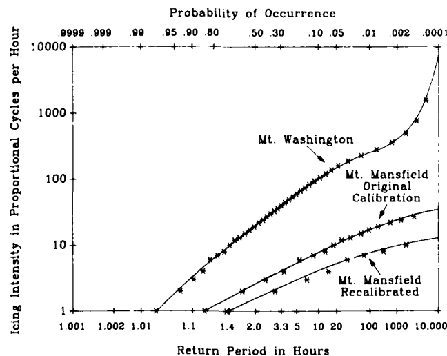
Figure 15. Return probabilities for hourly icing intensity in proportional Rosemount deicing cycles per hour for hours of icing of coincident record period.
