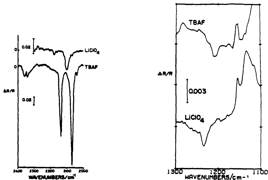
Fig. 3. SNIFTIRS difference spectrum in C≡N stretching region for reduction of TCNE to TCNE 2- at a platinum electrode. Solution thickness ca 50 μm. Same solutions as Fig. 1. Top spectrum: 0.1 M LiClO 4 as supporting electrolyte, potential modulated from +0.5 V to -1.2 V. Bottom spectrum: 0.1 M TBAF as supporting electrolyte, potential modulated from -0.5 V to -2.0 V.
