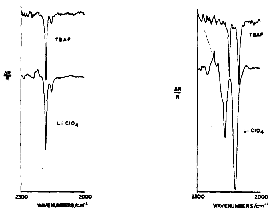
Fig. 7. SNIFTIRS difference spectrum in C\equiv N stretching region for reduction of TCNQ to TCNQ •- at a platinum electrode. Solution thickness ca 50 \mu\text{m} . Solutions contained TCNQ (5 mM) in acetonitrile with 0.1 M LiClO 4 (top spectrum) and 0.1 M TBAF (bottom spectrum) as supporting electrolyte. Potential modulated from +0.4 V to -0.2 V (vs. Ag/0.01 M Ag + reference).
