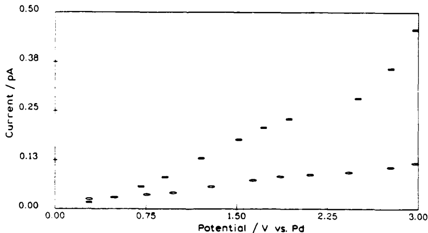
Fig. 3. Ultramicroelectrode response vs. potential applied for the injection of 1 \mu\text{l} of a solution 50% in toluene and 50% in triethylamine. (□) Toluene response, (O) triethylamine response.
