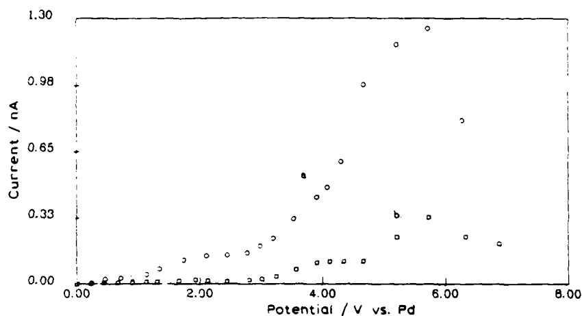
Fig. 4. Ultramicroelectrode response vs. potential applied for the injection of 1 \mu\text{l} of a solution of 30% cyclohexanone in triethylamine. (□) triethylamine response.
