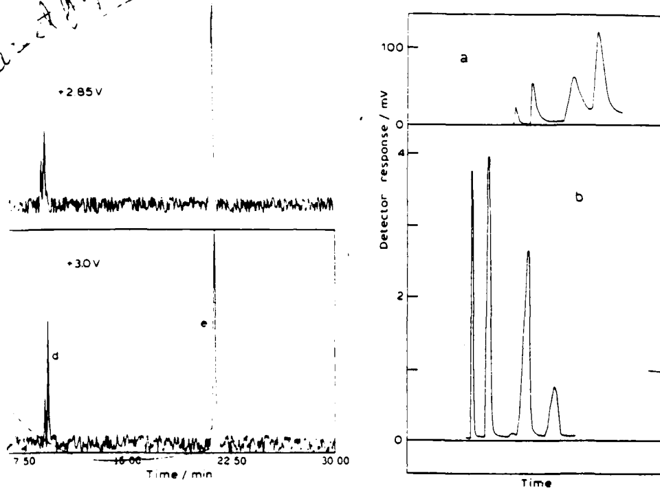
CONTAINING Fig. 5. (a) Ultramicroelectrode detector, (b) thermal conductivity detector responses after the injection of a solution containing 30% toluene, 46% (v/v) o -xylene. The peaks from left to right correspond to acetone, toluene, o -xylene, and cyclohexanone, respectively. Applied potential was +3.0 V. The total time is 16 min.
