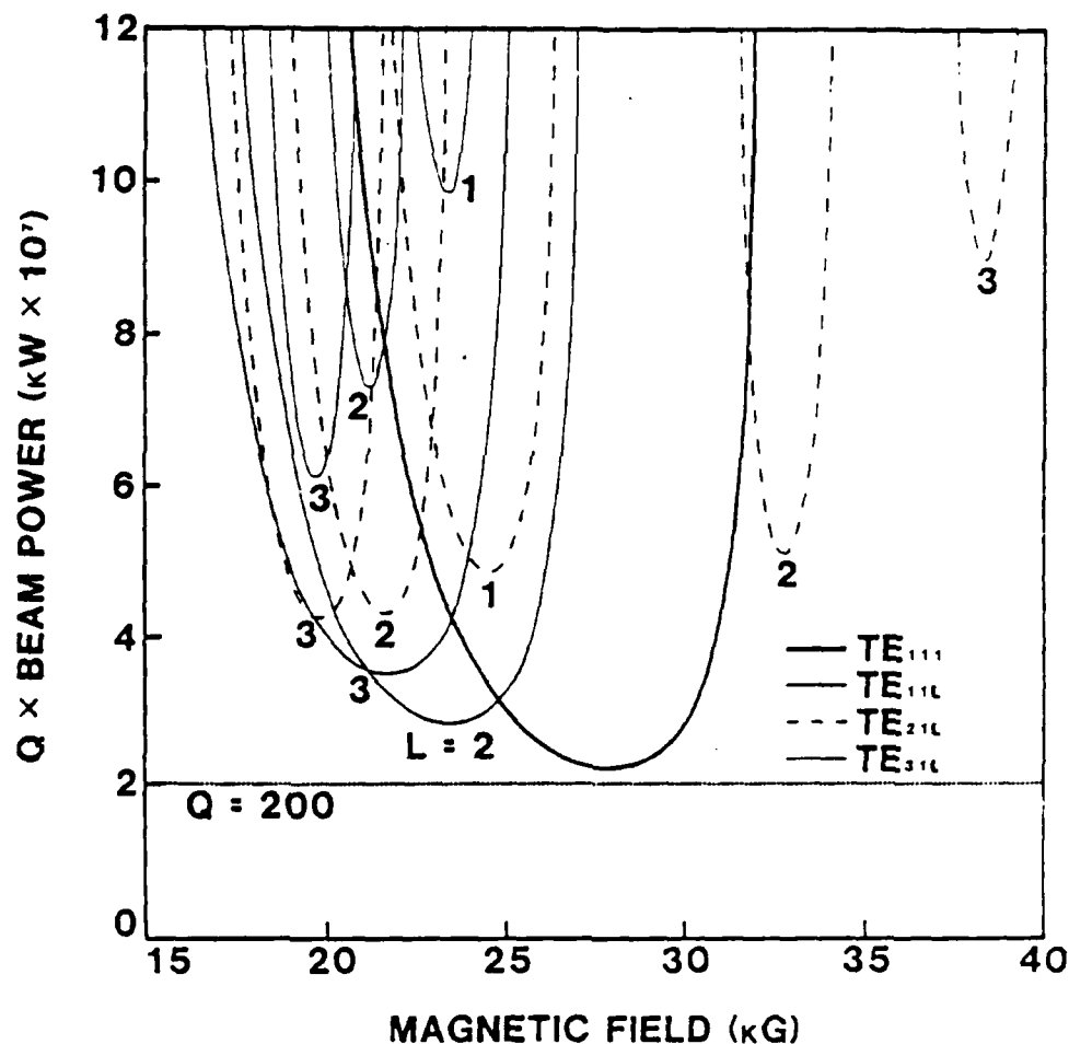
Fig. 2. Scan of Q \times threshold beam power versus magnetic field for the TE_{111} mode and competing modes in the bunching cavity. The calculations assume a sinusoidal axial RF field profile with L/\lambda=2 , circular polarization, and \alpha=0.75 . The TE_{11} modes interact at the first harmonic, the TE_{21} modes interact at the second harmonic, and the TE_{31} modes interact at the third harmonic.
