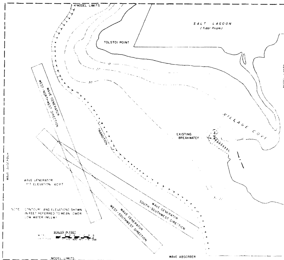
Figure 3. Model layout
