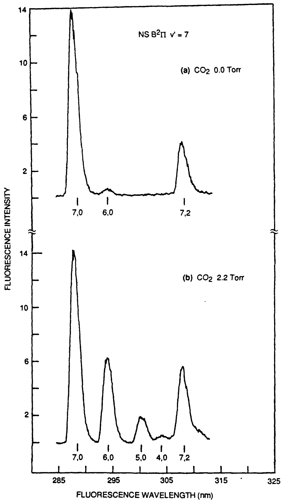
Figure 5. Wavelength-resolved fluorescence following excitation to v' = 7 with and without added CO 2 collider.
