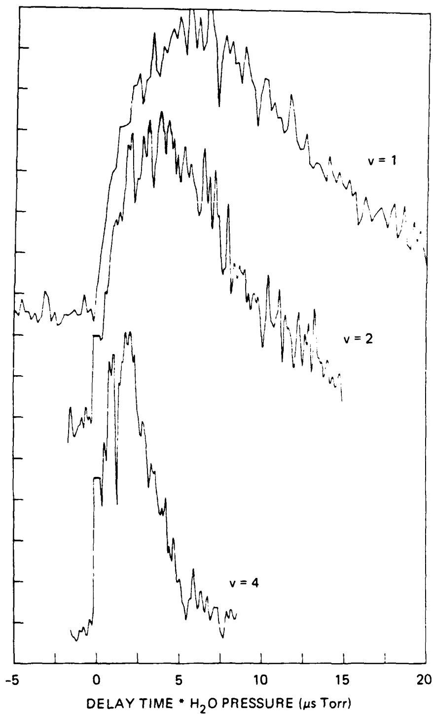
Figure 1. Time-dependent populations of vibrational levels v'' = 1, 2, and 4 in \text{OH } X^2\Pi_i , following quenching of A^2\Sigma^+, v' = 0 , by collisions with \text{H}_2\text{O} .
