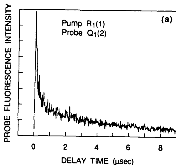
Figure 2. LIF exciting from OH X^2\Pi_i , v^* = 2 , as a function of delay time after initial state preparation by overtone pumping. The R 1 (1) infrared line of the 2-0 vibrational band is the pump transition. The ultraviolet LIF monitors population in the prepared F 1 (2) level (a and b) and in the collisional filling of F 1 (3) (c) and F 1 (4) (d) levels.
