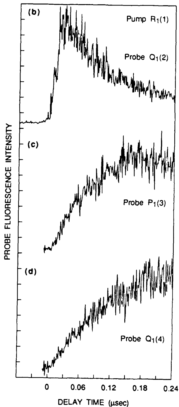
Figure 2. LIF exciting from OH X^2\Pi_i , v^* = 2 , as a function of delay time after initial state preparation by overtone pumping. The R 1 (1) infrared line of the 2-0 vibrational band is the pump transition. The ultraviolet LIF monitors population in the prepared F 1 (2) level (a and b) and in the collisional filling of F 1 (3) (c) and F 1 (4) (d) levels.
