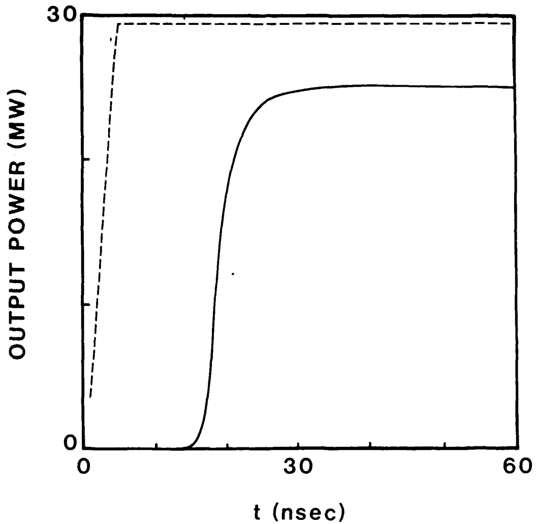
Fig. 4. Results of the time-dependent CARM oscillator code show that the 70 nsec pulse should be sufficient to drive the interaction to saturation. The dashed line represents the voltage waveform.
