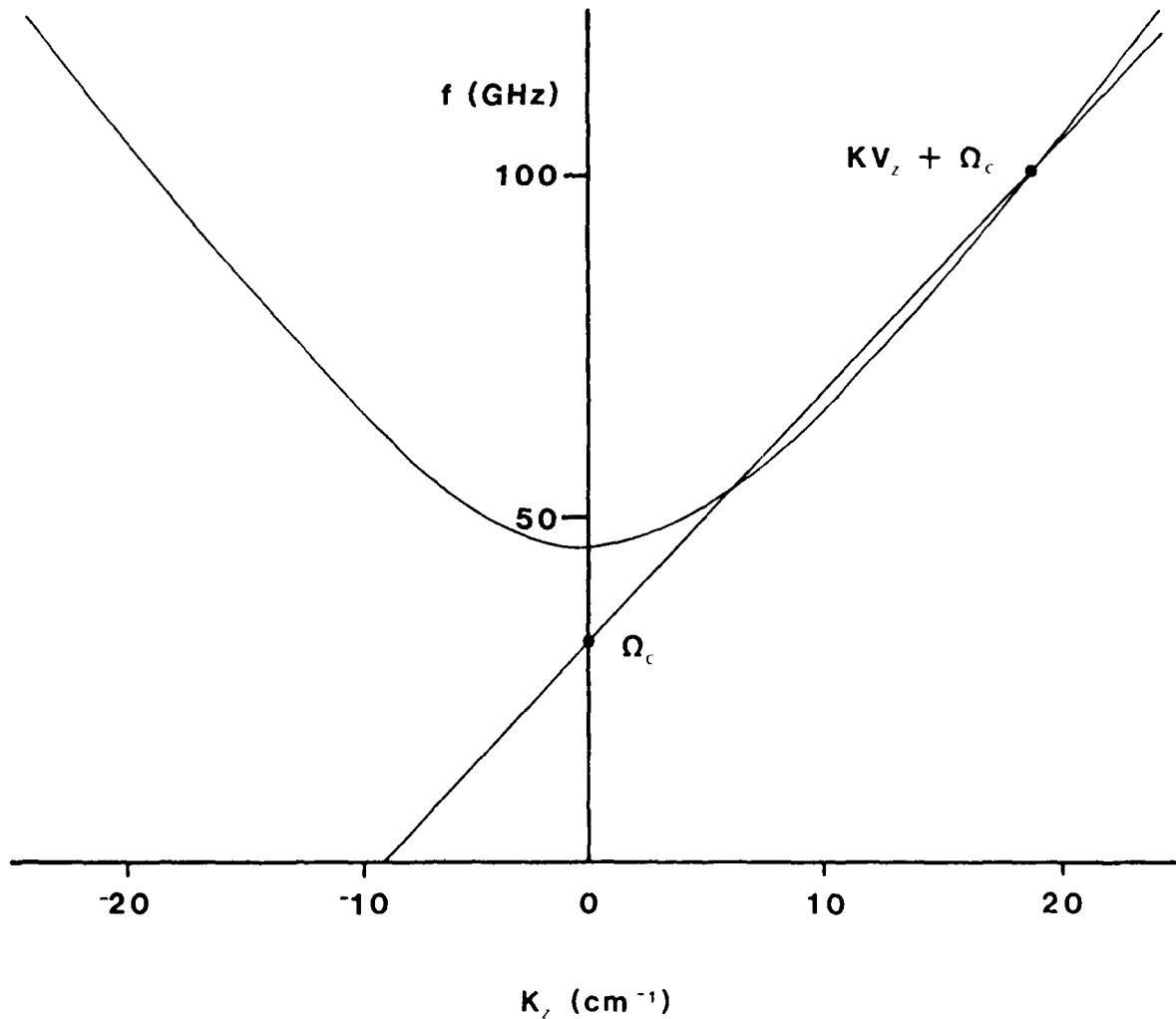
Fig. 1. The dispersion relation for the NRL 100 GHz. CARM experiment. The high frequency intersection of the electron beam line with the TE_{61} waveguide dispersion relation is the CARM operating regime. The lower frequency intersection is a competing gyrotron mode.
