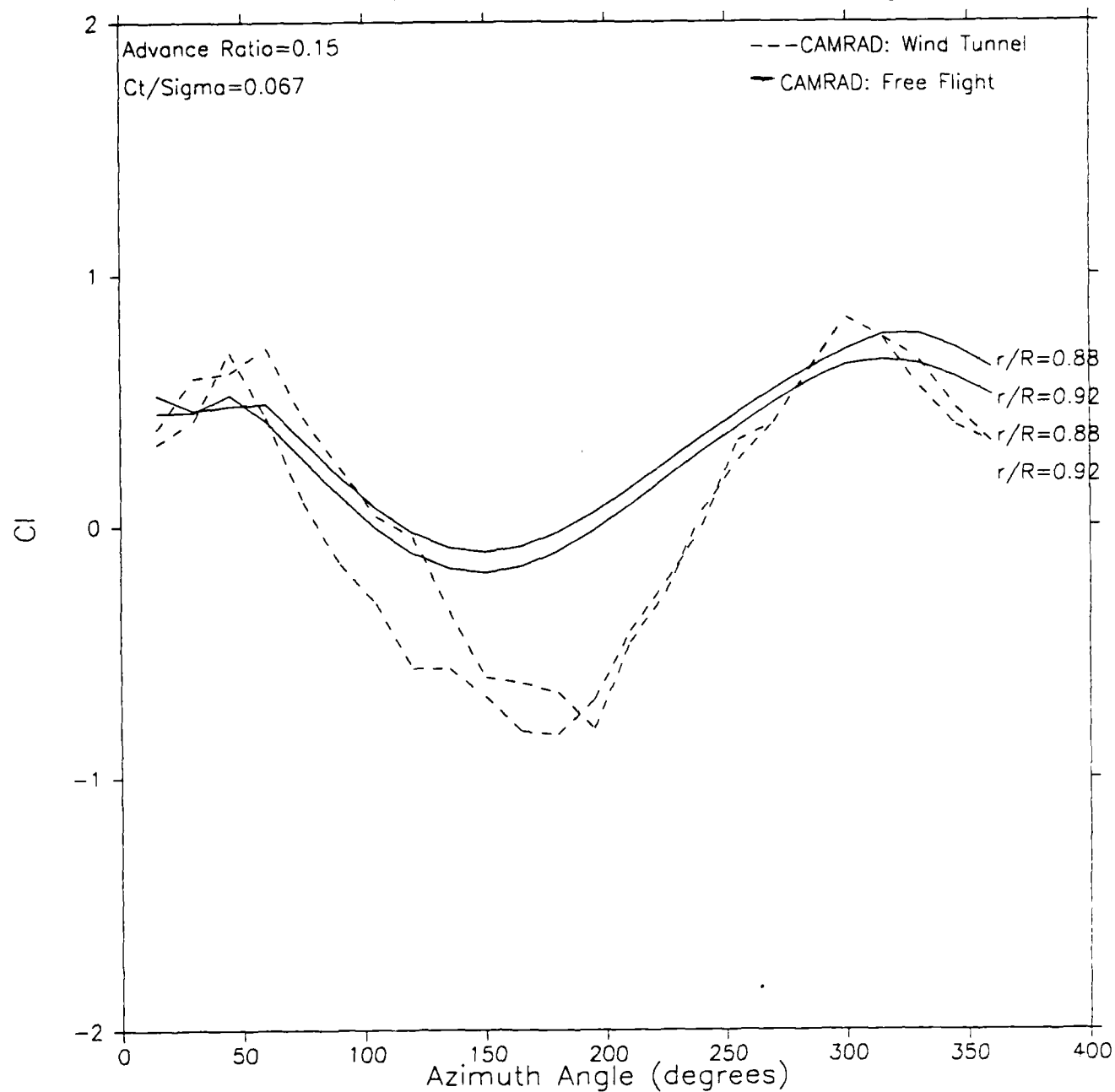
FIGURE 22: Lift Coefficient vs Azimuth Angle
