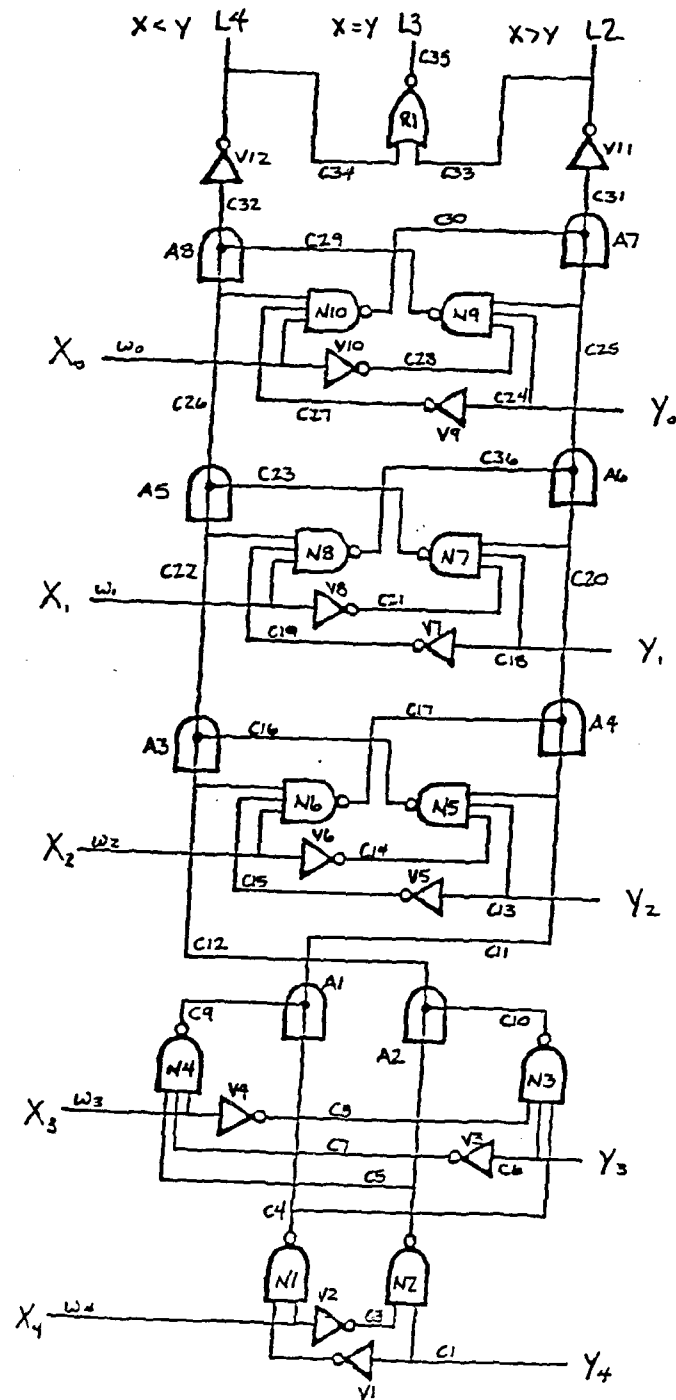
Figure 5. 5-Bit Comparator
