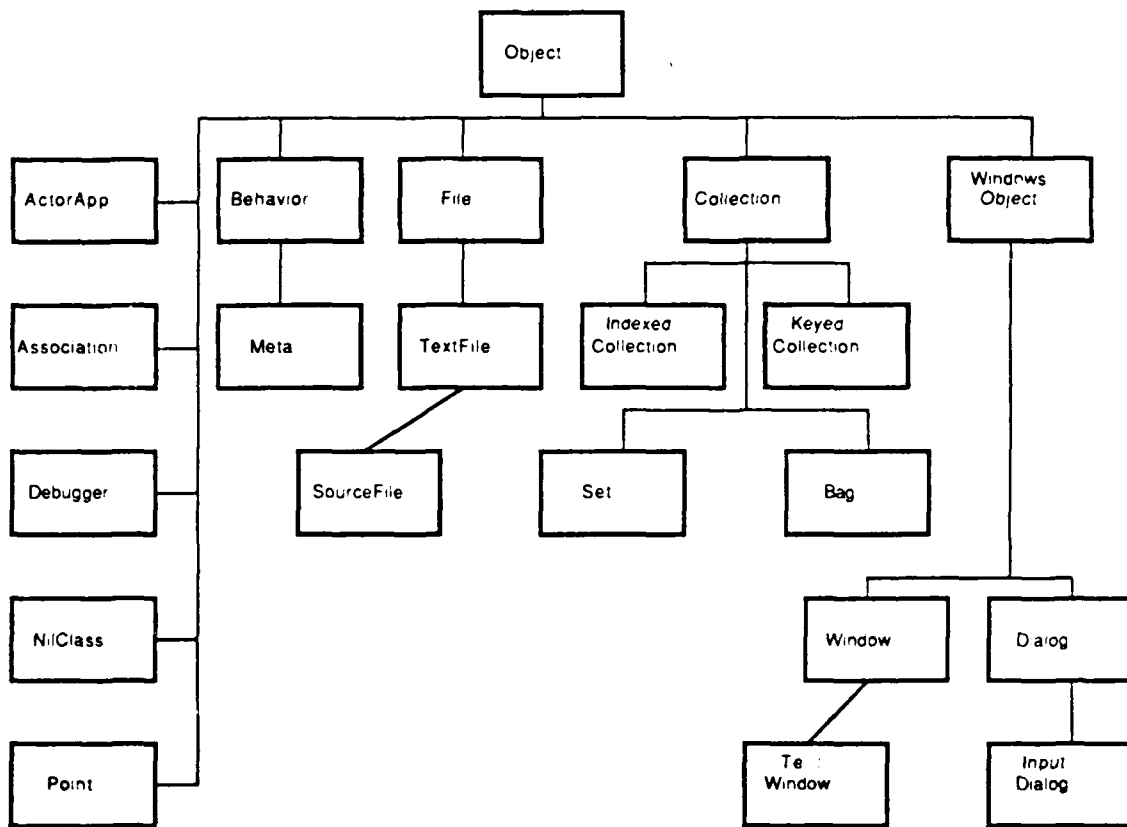
Figure 2. The Actor Tree of Predefined Classes
