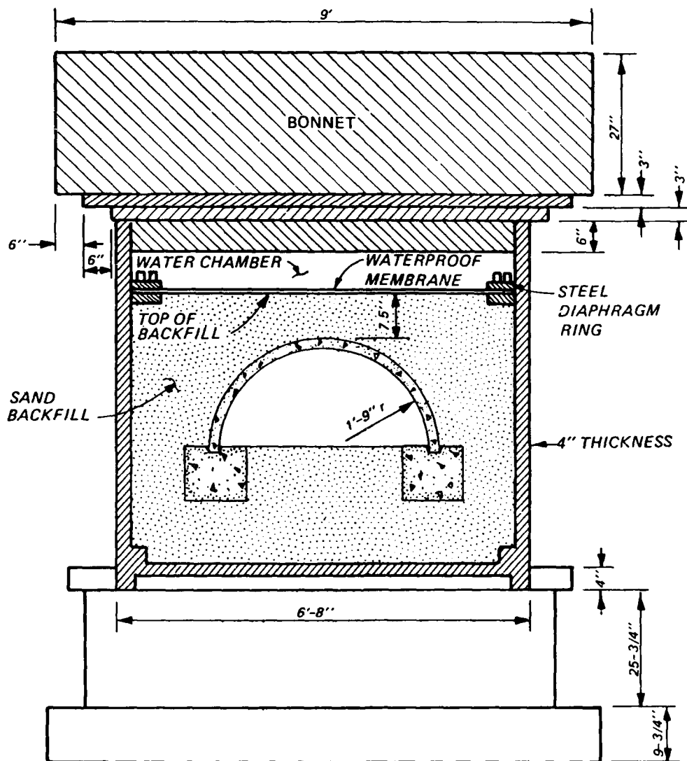
Figure 10. Test configuration.
