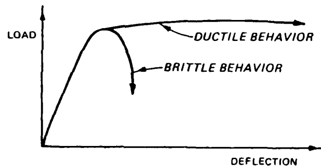
Figure 60. Load-deflection behavior of a flexural member.
