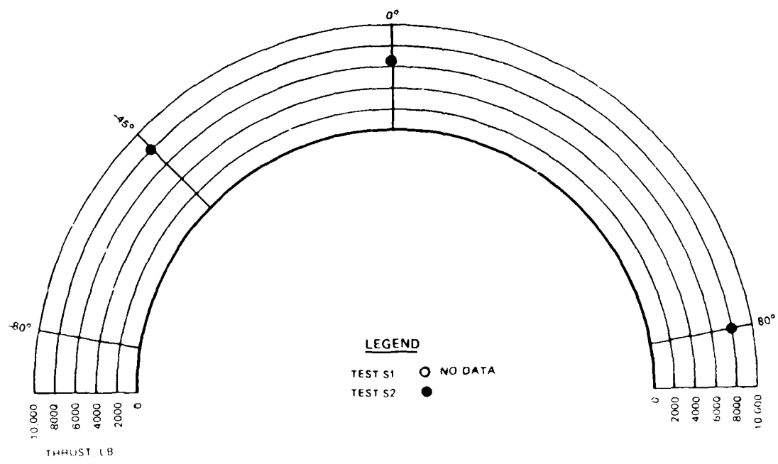
Figure 53. Experimental thrust in arch ring at water pressure ( WP' = 500 and 600 psi).
