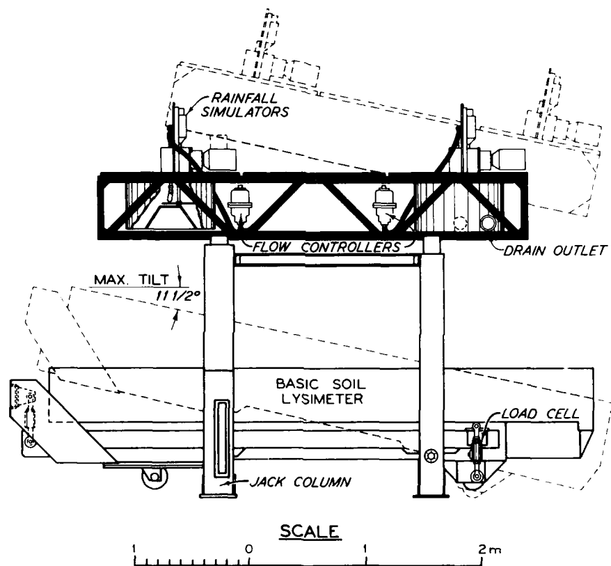
Figure 1. The WES Rainfall Simulator, Lysimeter System
