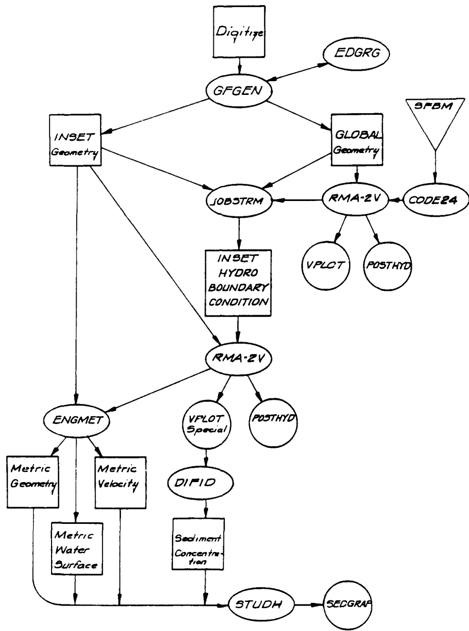
Figure 3. Flowchart of programs
