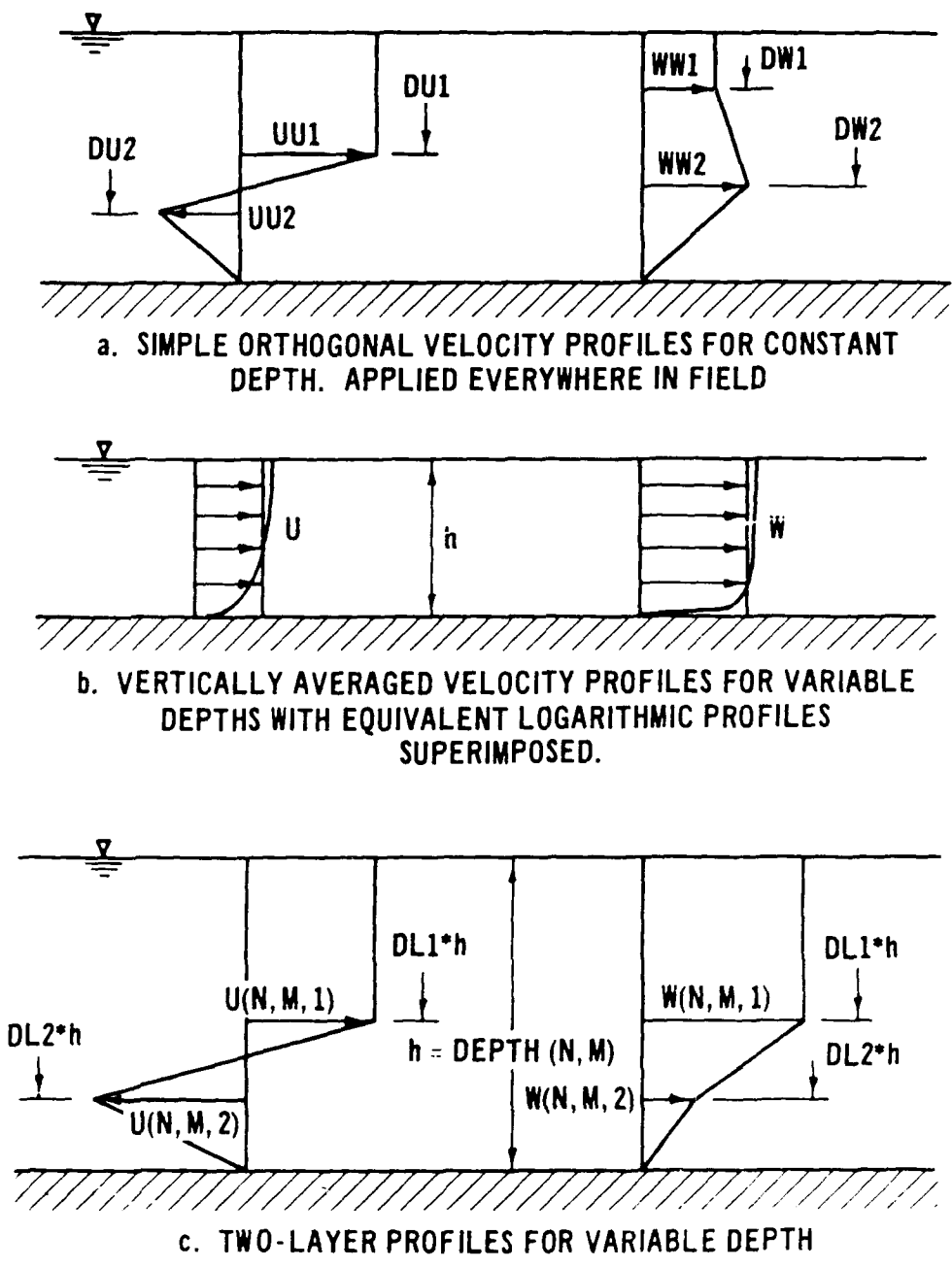
Figure B3. Illustration of the various velocity profiles available for use in models (from Brandsma and Divoky 1976)
