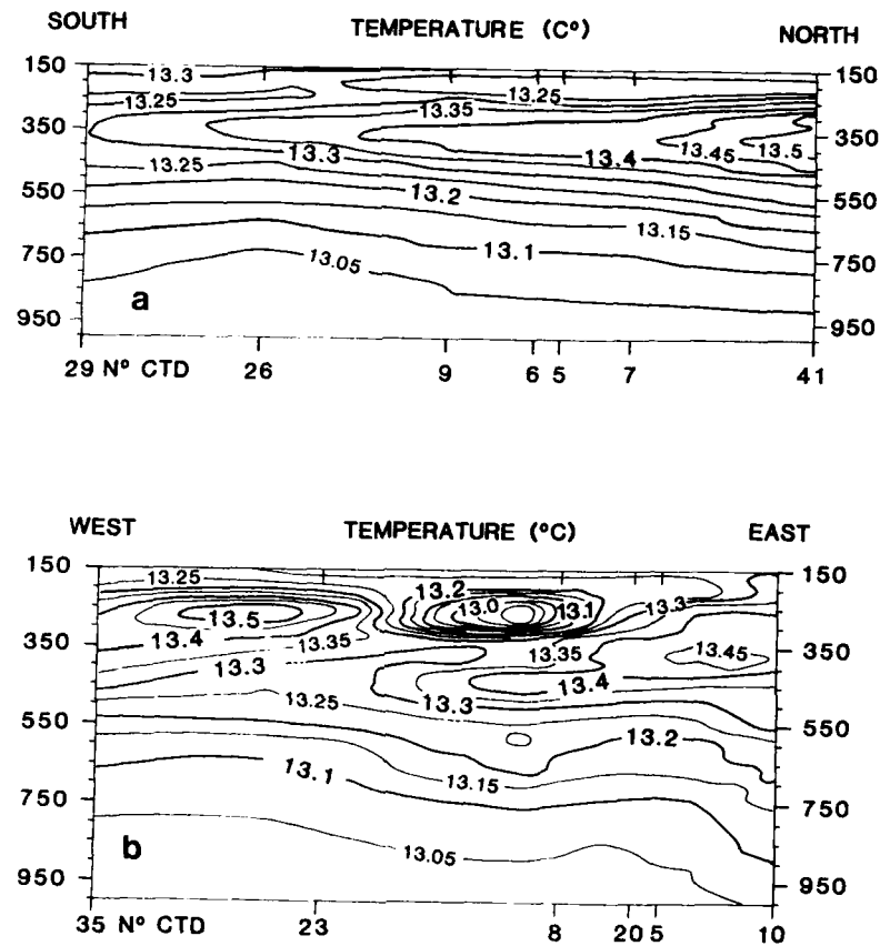
Fig. 12. Vertical temperature sections for the intermediate 150–1000 m layer: (a) south-north and (b) west-east.
