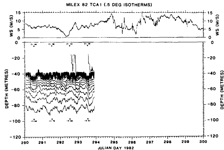
Fig. 15c. Temperature contours from thermistor chain A1 for days 290-300. Contour intervals are very 0.5°C and positions with temperatures of uppermost and lowermost thermistors are indicated by a star symbol every 24 h. Wind speed is plotted to indicate wind forcing on the thermocline.
