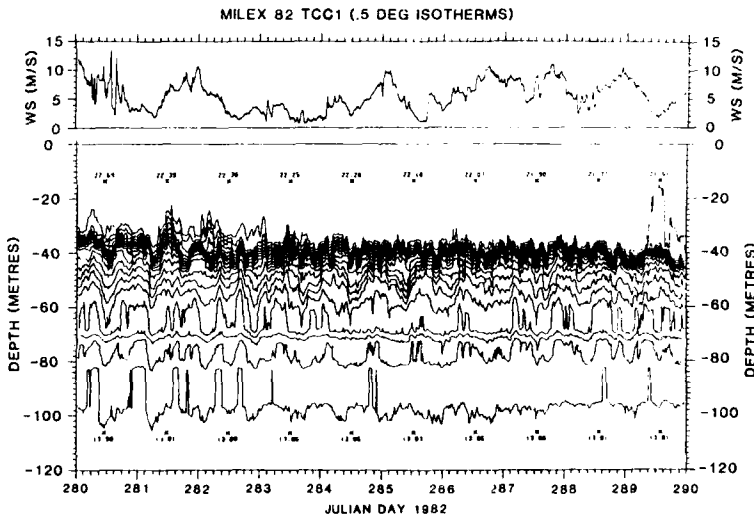
Fig. 17b. Temperature contours from thermistor chain C1 for days 280–290. Contour intervals are very 0.5^{\circ}\text{C} and positions with temperatures for uppermost and lowermost thermistors are indicated with a star symbol every 24 h. Wind speed is plotted to indicate wind forcing on the thermocline.
