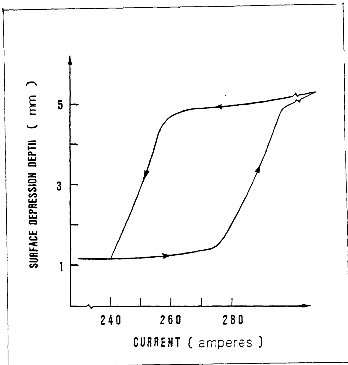
Figure 13. Plot of surface depression versus current observed by Lim. [1]
