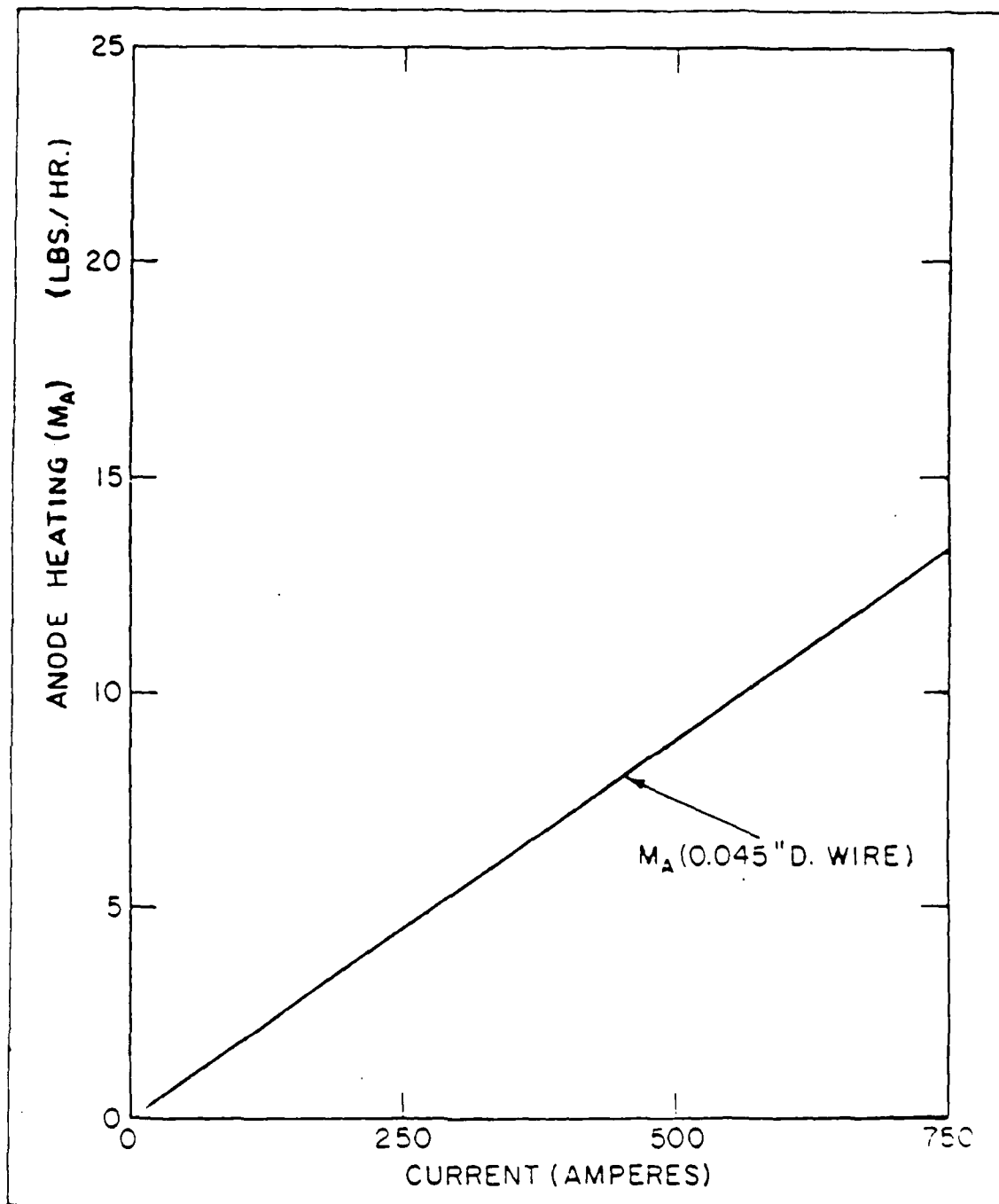
Figure 5. Dependence of melting rate due to anode heating on the magnitude of welding current.[4]
