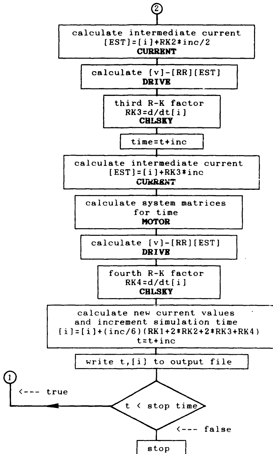
Figure 3-1.(cont.) FORTRAN simulation program flowchart.
