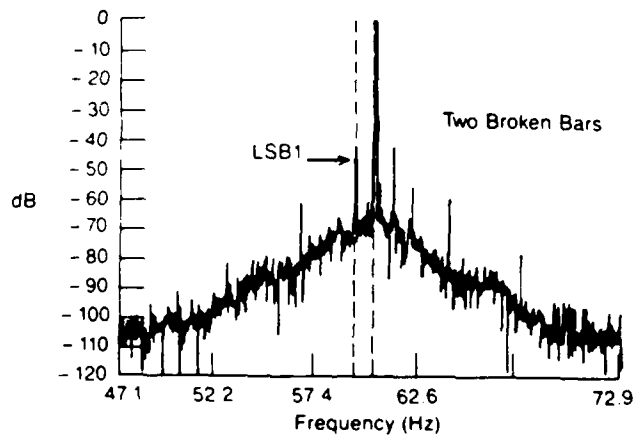
Figure 1-4. BBD experimental results for s=0.01 [7].
