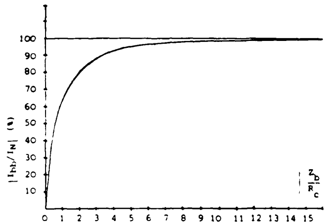
Figure 4-11. Ratio of current in a broken bar to a "healthy" bar [9].
