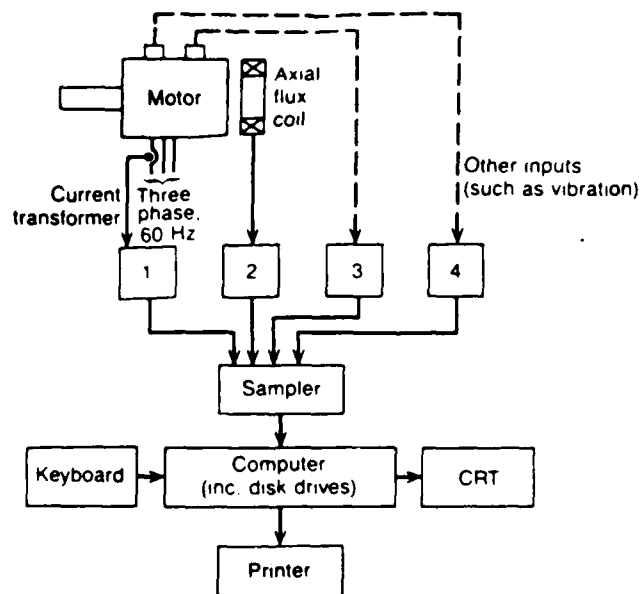
Figure 1-3. BBD one-line diagram [7].
