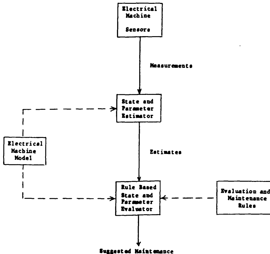
Figure 1-1. Proposed failure analysis system [5].
