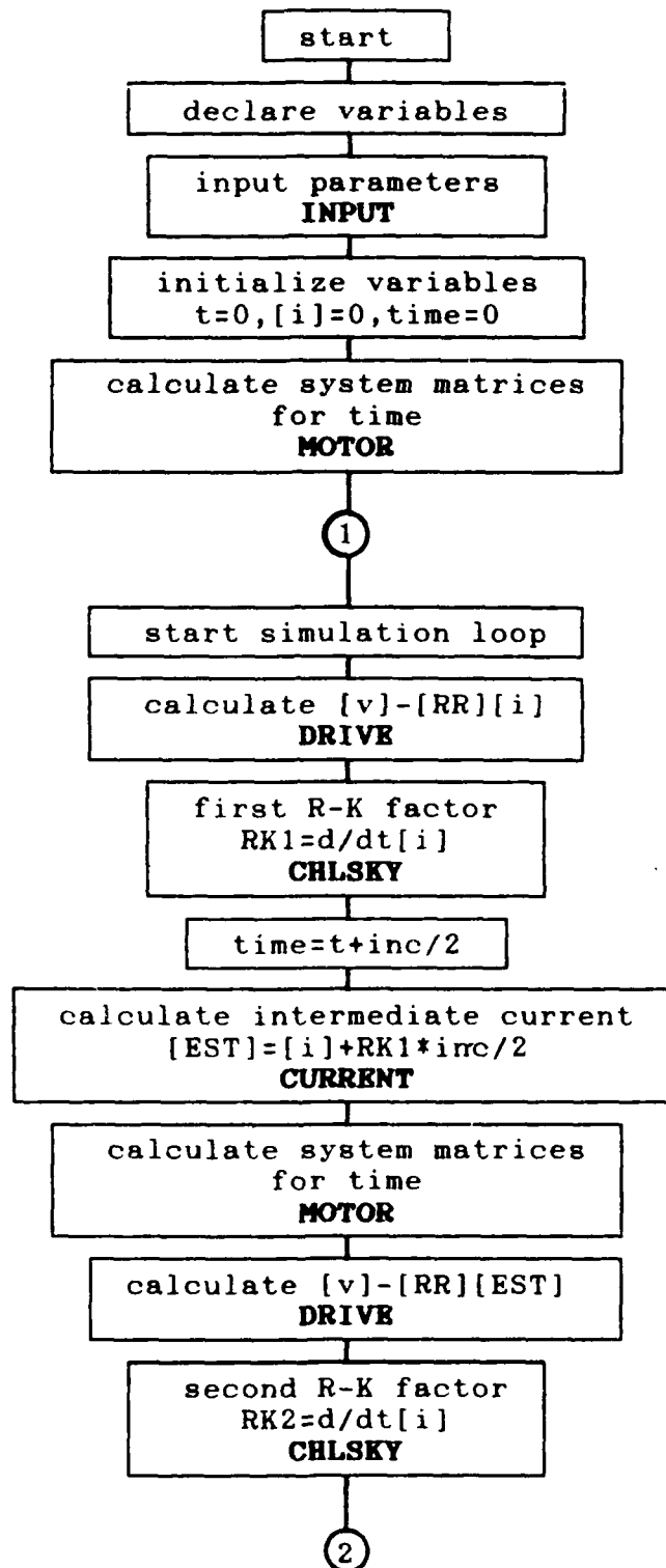
Figure 3-1. FORTRAN simulation program flowchart.
