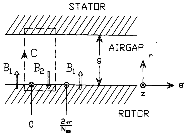
Figure 2-5. Integration contour on rotor.
