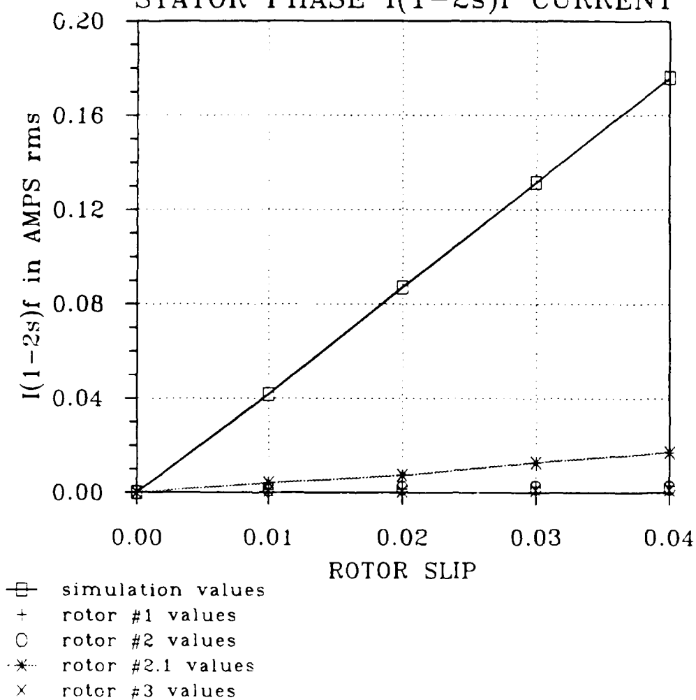
Figure 4-20. Simulation and experimental results I(1-2s)f .
