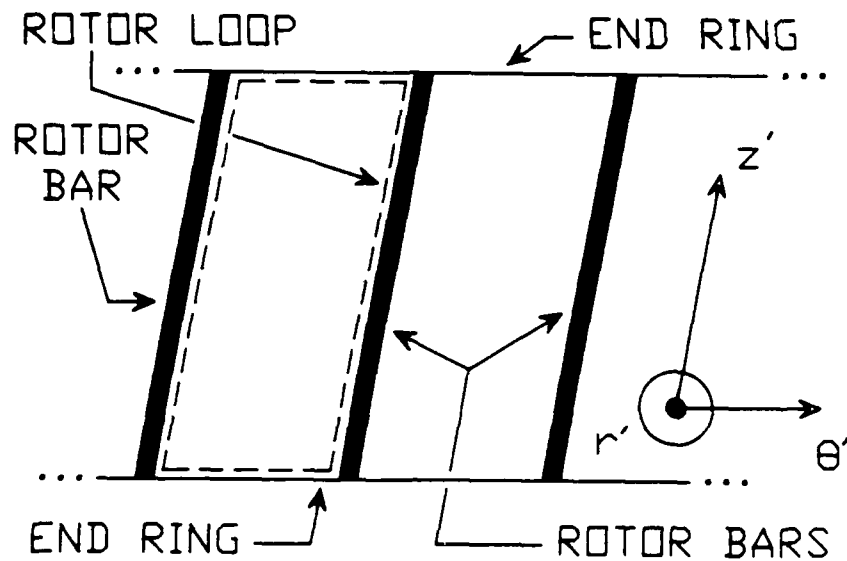
Figure 2-2. Rotor loop description.
