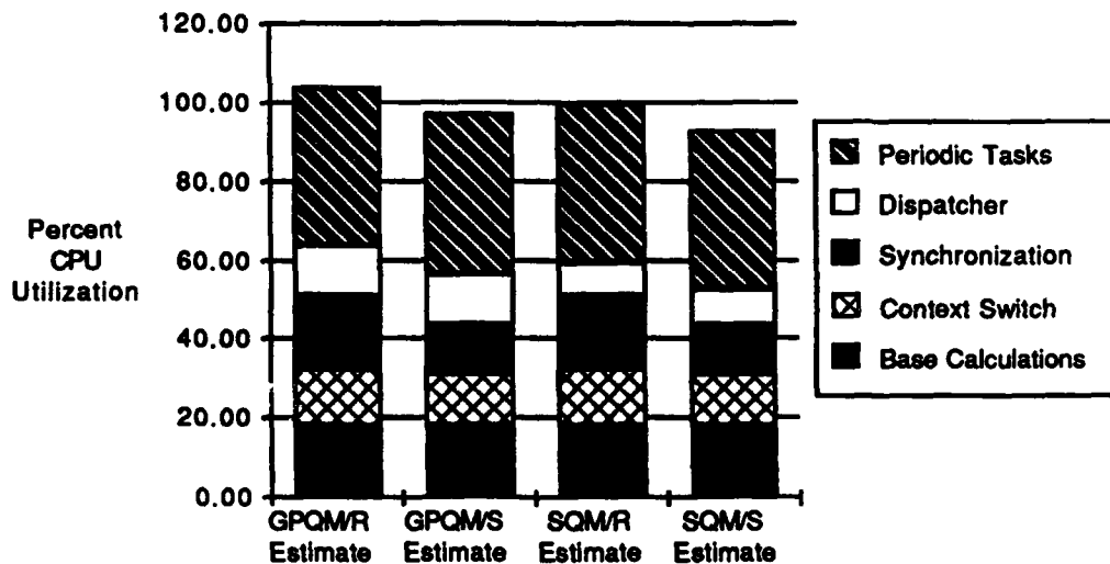
Figure 4-1: Rendezvous Versus Semaphore Comparison
