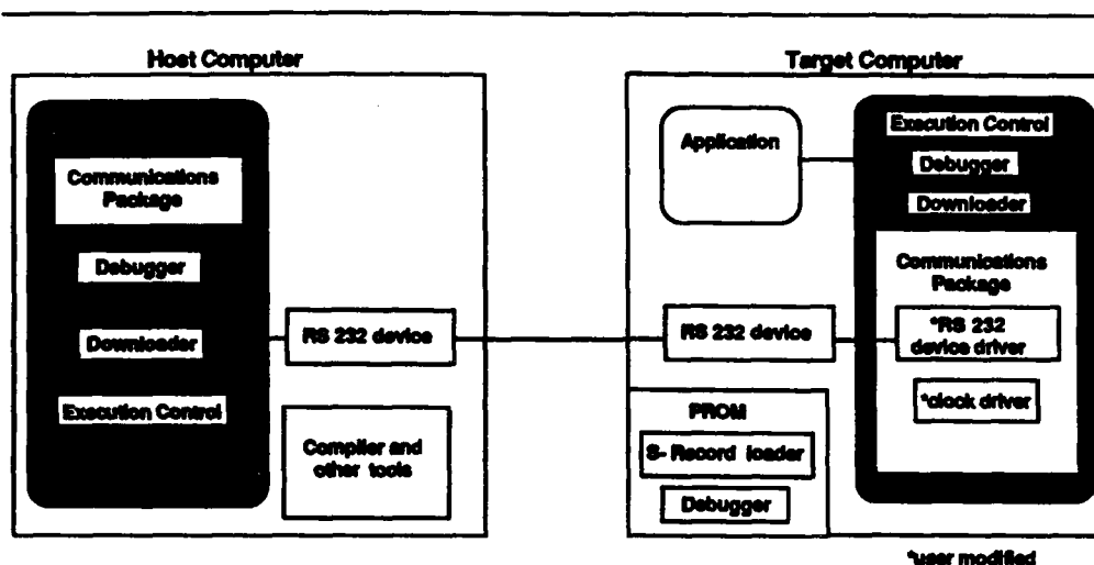
Figure 2-1: Typical Host Computer/Target Computer Configuration
