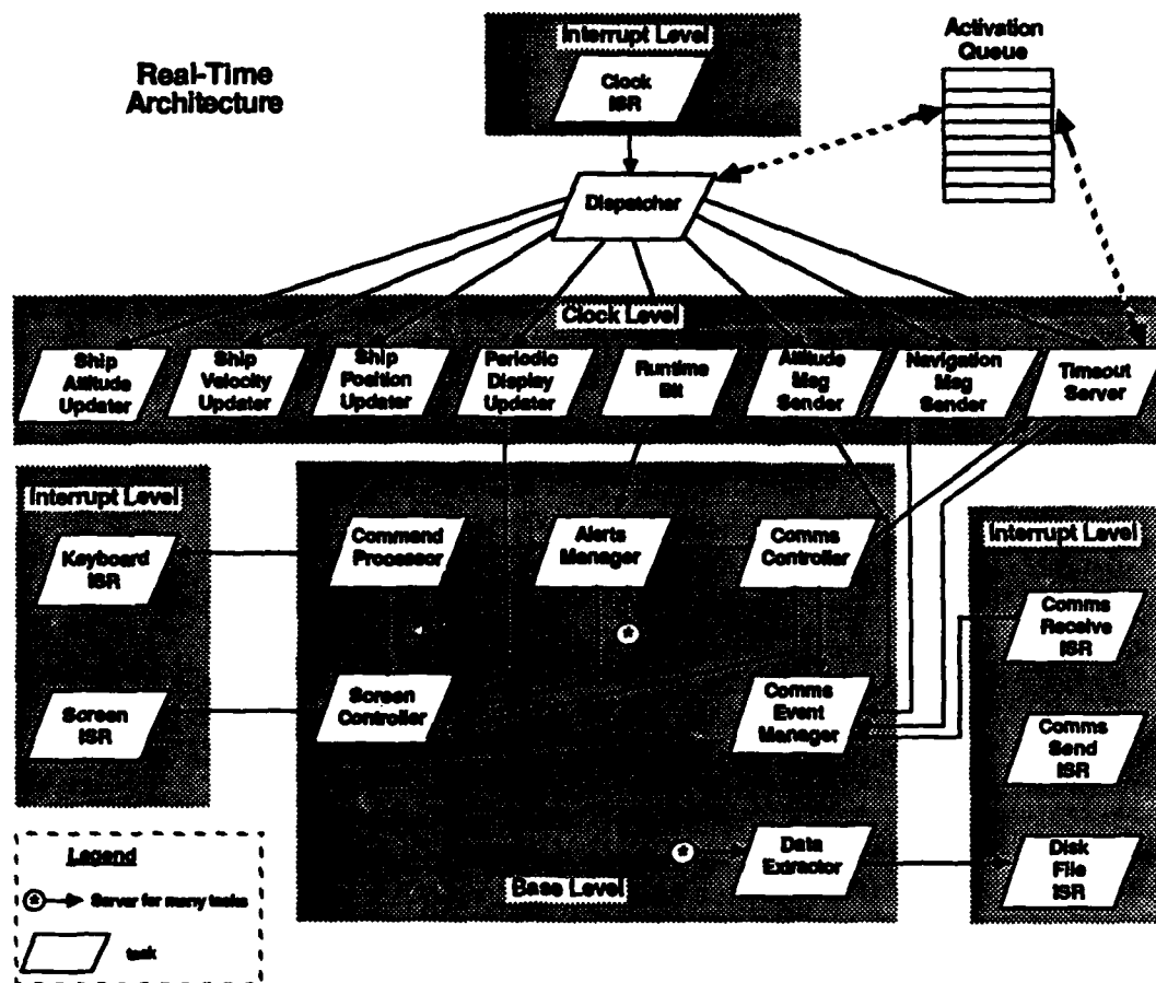
Figure 5-2: Real-Time Architecture
