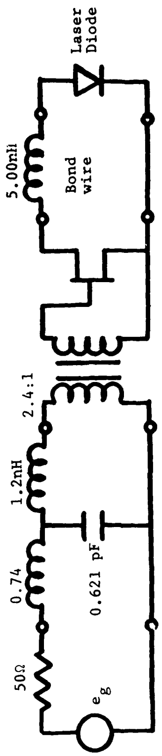
Figure 15: Realization, example 3
