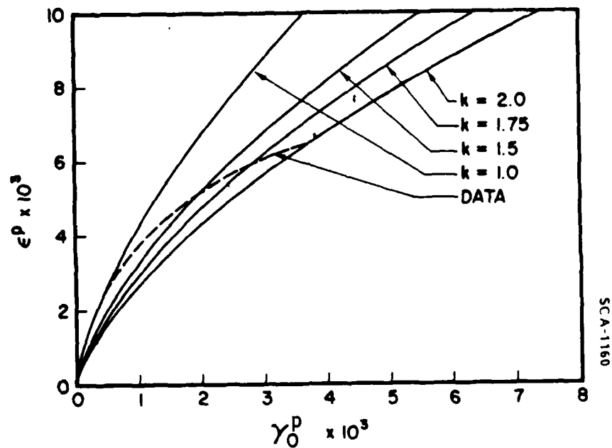
Figure 9.2 Shear-volumetric coupling at a constant hydrostatic pressure of 8 ksi. Data are from Test 4-11 Reference [9.1].
