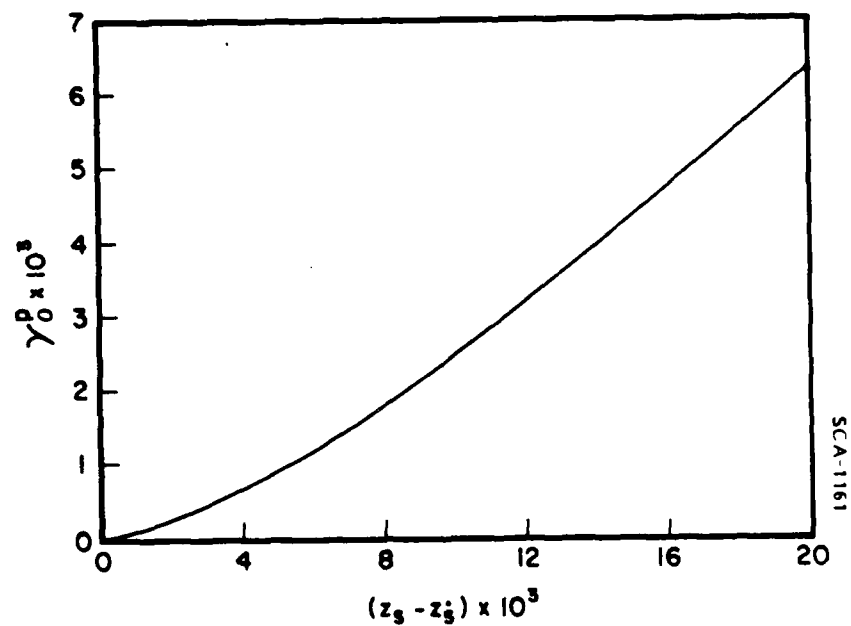
Figure 9.3 Dependence of \gamma_0^p on z_s - z_s^* predicted by Eqs. (9-18) and (9-19) for shear at a constant pressure of 8 ksi.
