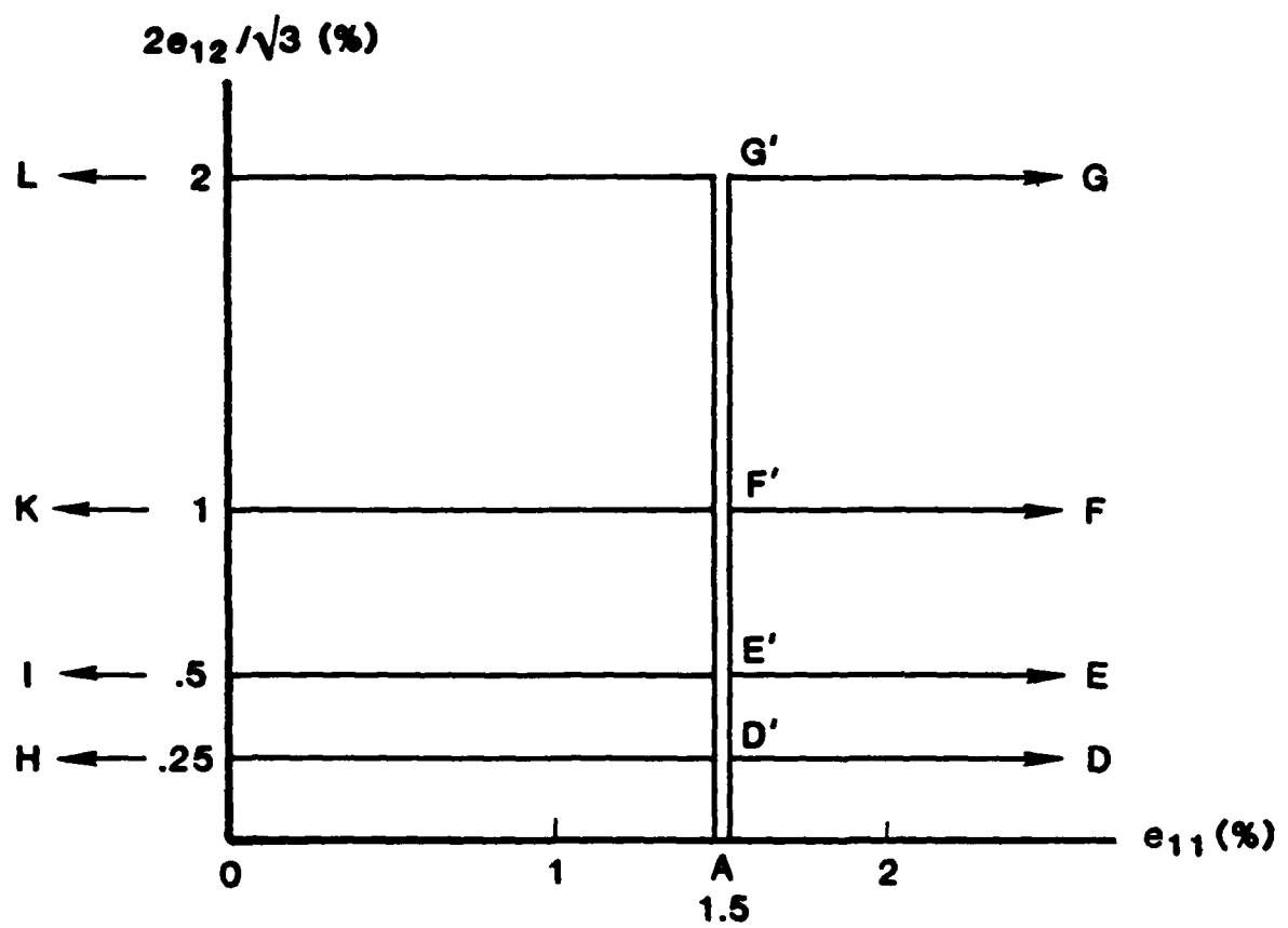
Figure 3.19. Map of experimental strain paths.
