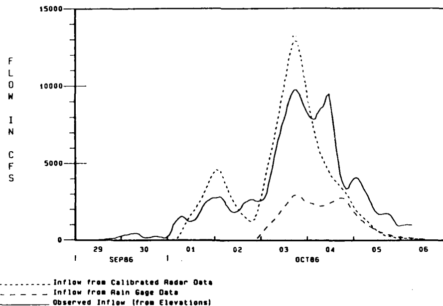
Figure 3. Computed and Observed Inflows (observed inflow calculated from reservoir elevations).
