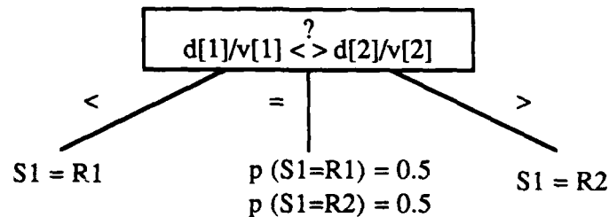
Figure 6.3 One Comparison Using Algorithm 2
