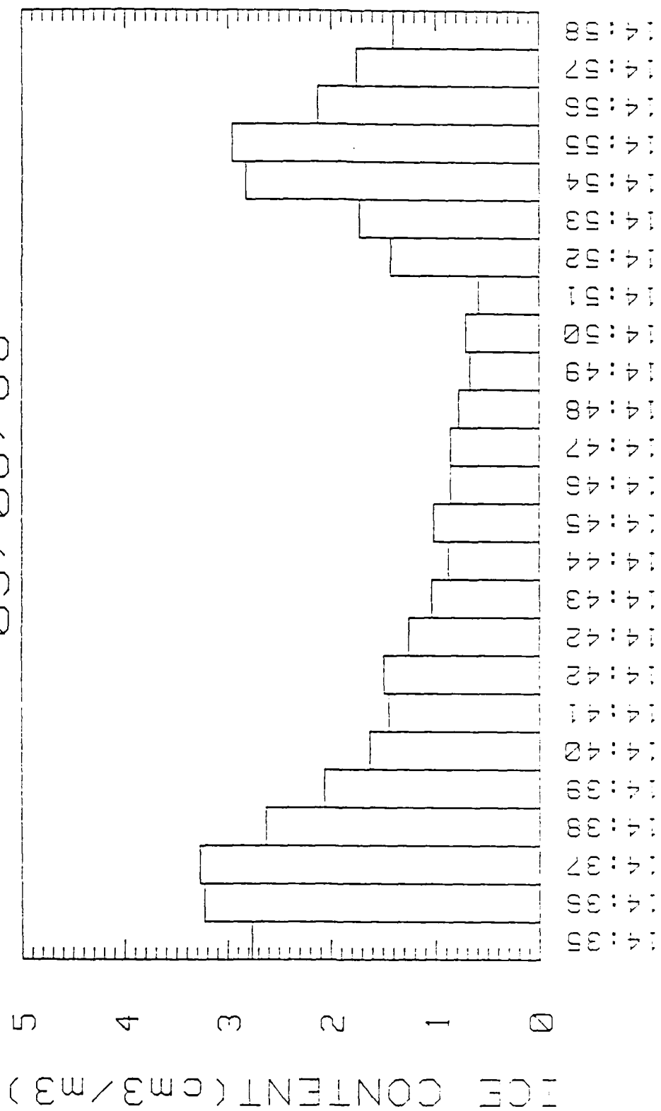
Fig. 13 Ice content computed from size distributions.
