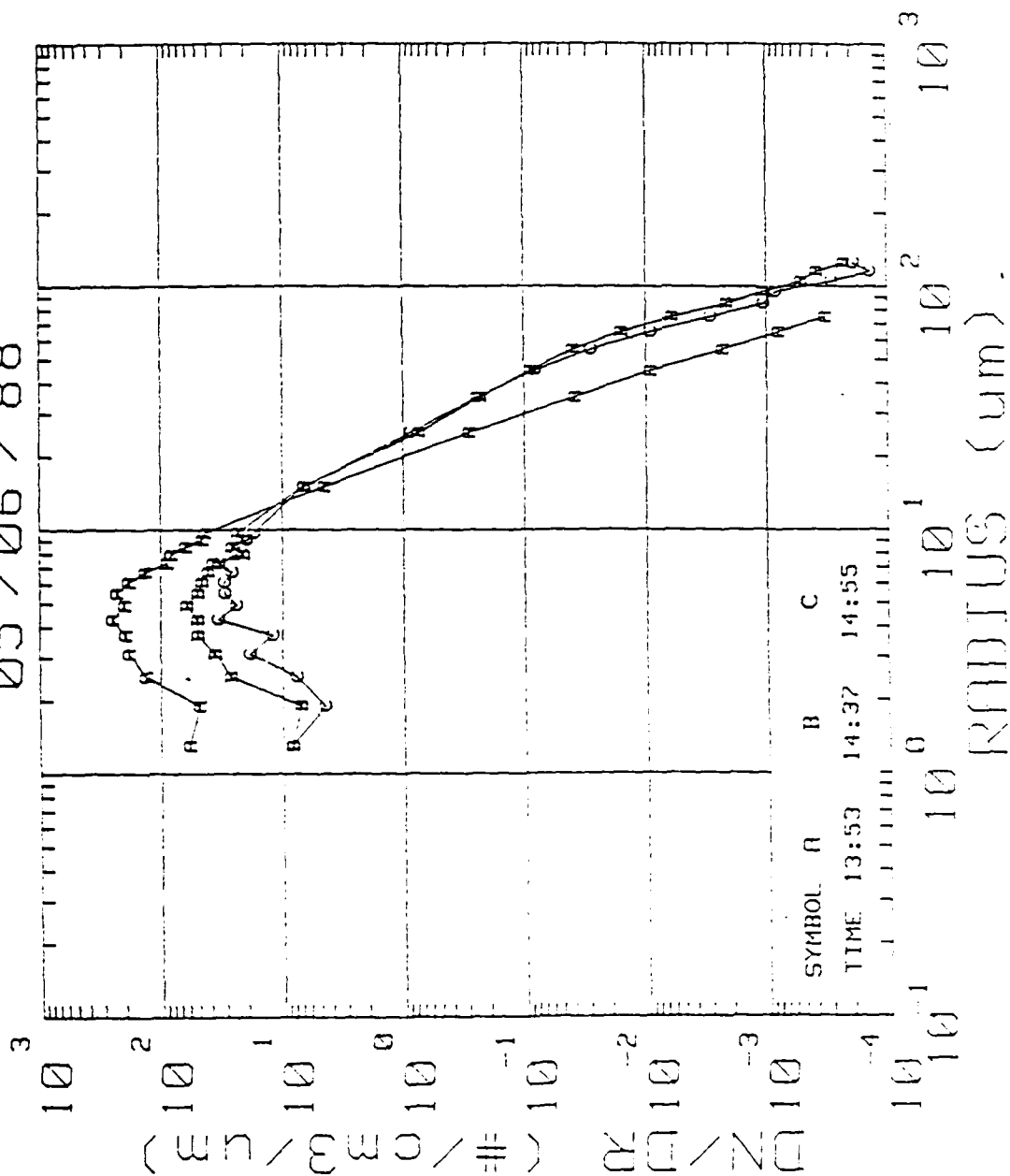
Fig. 15 Size distributions from the three ice fogs.
