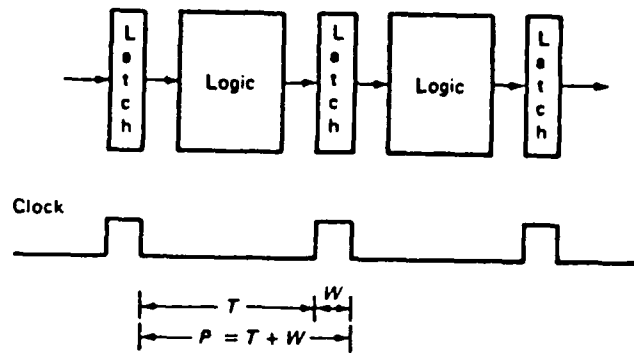
Figure 3.1 Two Stages and Pipeline Clock
