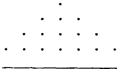
Figure 4.4 Wallace Tree Partial Products
