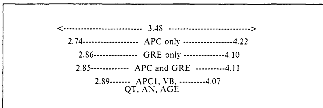
Figure 3. Forecast Intervals--Division 06
