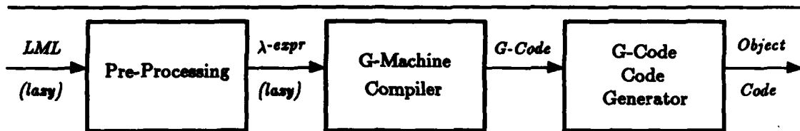
Figure 2.6: Abstract Machine Lazy Compilation: the LML/G-Machine Compiler
