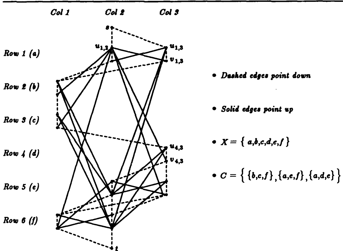
Figure 5.7: Construction Reducing X3C to CCAS
