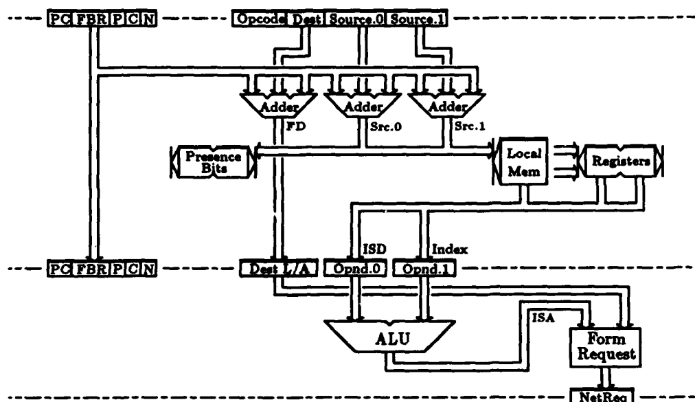
Figure 3-15: Flow of Data for the LOAD Instruction
