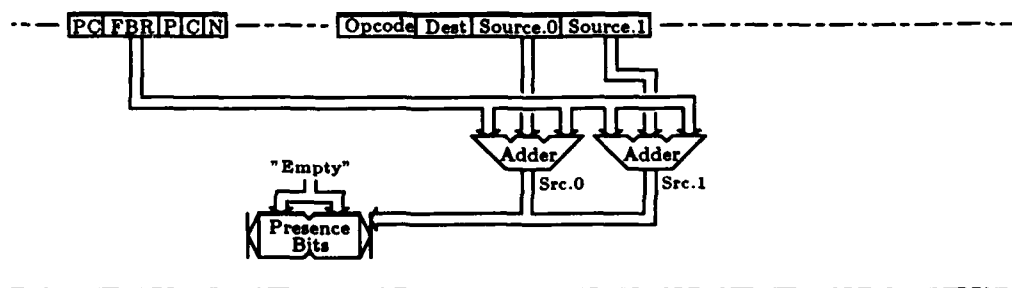
Figure 3-17: Flow of Data for the RSTN Instruction
