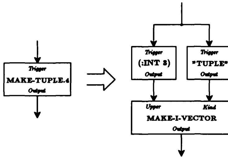
Figure 4-9: Rewriting MAKE-TUPLE.4
