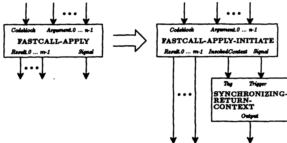
Figure 4-13: Rewriting FASTCALL-APPLY
