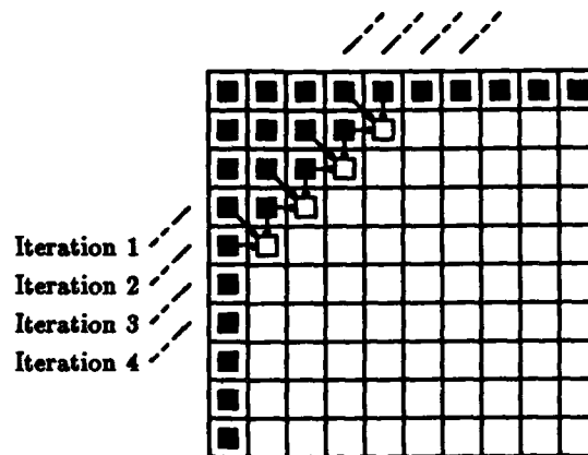
Figure 2-5: Dependences and Parallelism in WaveFront
