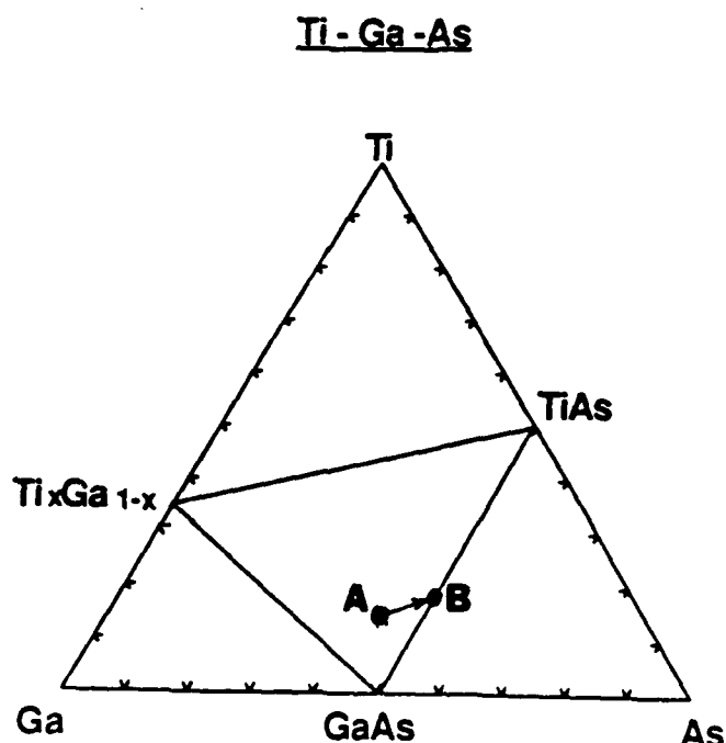
Figure 4 Partial Ti:Ga:As ternary phase diagram illustrating the shift in equilibrium from point A to B due to gallium outdiffusion.
