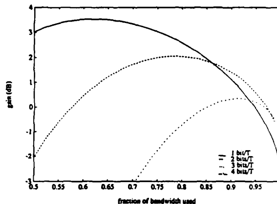
Figure 2 - Coding Gain vs. Fraction of 1/2T
