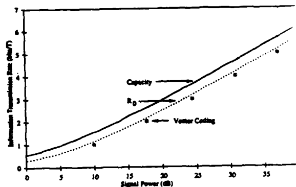
Figure 1b - R_0 for the 1-D channel
