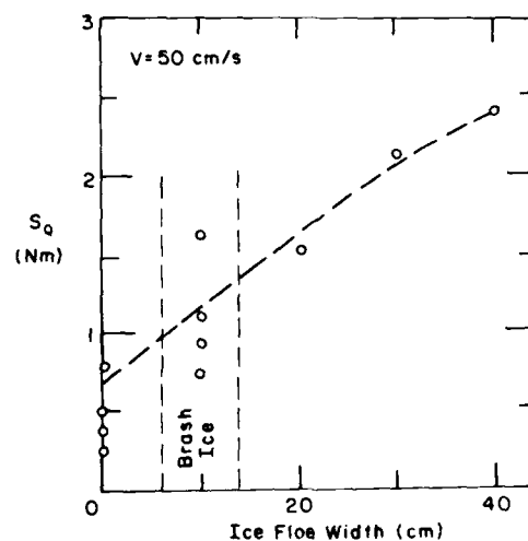
Figure 10. Effect of floe size on propeller performance (Tatinclaux 1987).
