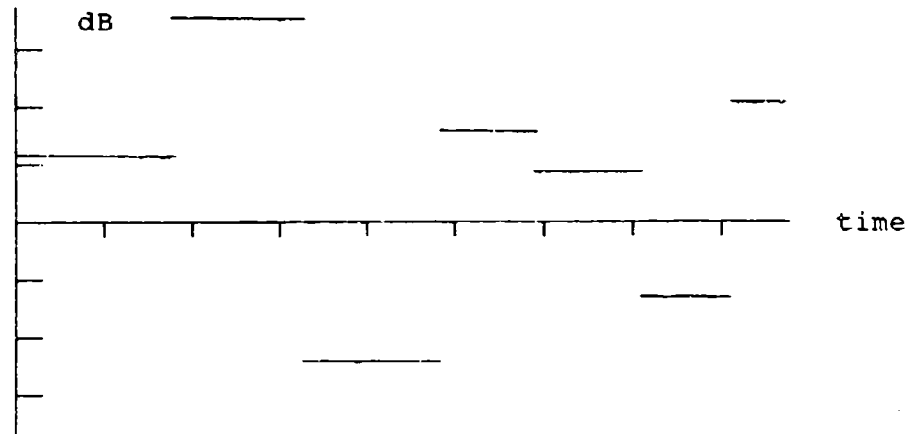
Figure 2. A time series representing a realization of a lambda-sigma jump process. On the plot, \sigma in dB equals one unit on the vertical axis and \tau equals one time unit on the horizontal axis.
