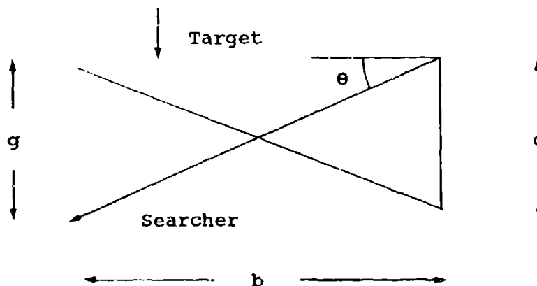
Figure 7. A barrier search track shown for a barrier established in front of the target. The track is shown in a reference system fixed relative to the earth.
