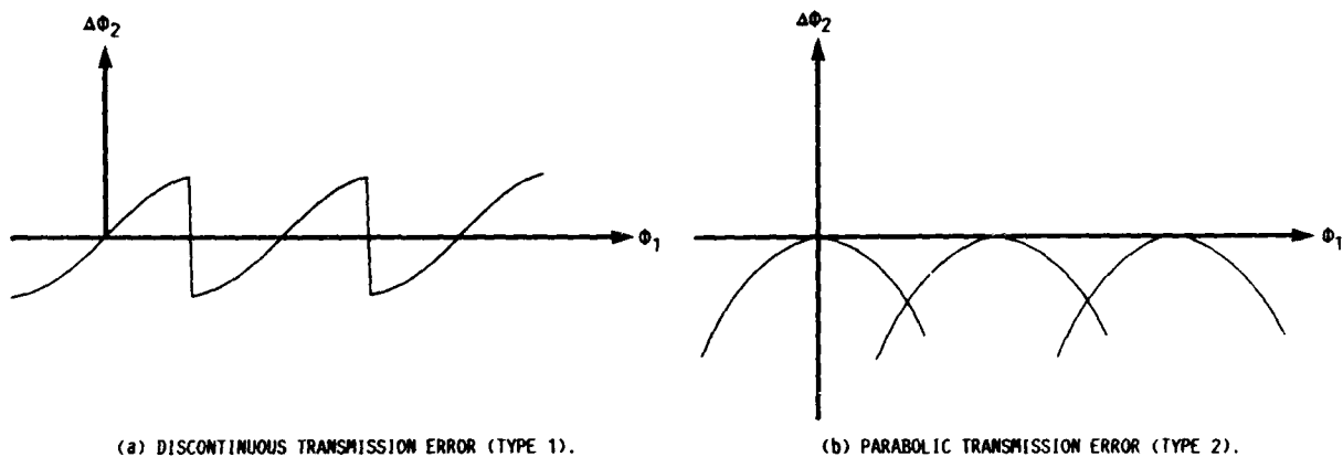
FIGURE 3. - TRANSMISSION ERRORS ( \Delta\phi_2 ) AS FUNCTION OF PINION ROTATION ( \phi_1 ).
