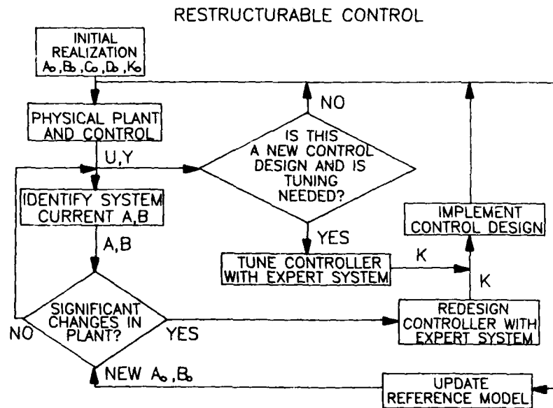
Figure 2 - Expert System Interaction with Overall System
