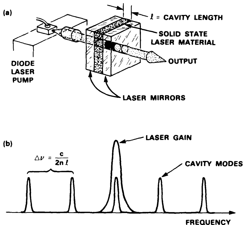
Figure 2-6. (a) Illustration of a diode pumped microcavity solid state laser. (b) Gain spectrum of a solid state medium shown superimposed on the cavity mode spacing of a microcavity laser to illustrate why single-frequency operation occurs.
