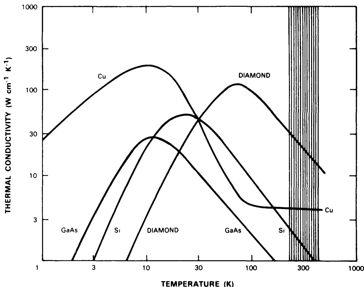
Figure 4-3. Thermal conductivities of several solids as a function of temperature. The vertical gray band around 300 K represents the temperature range from -25 to 125°C. The thermal conductivity of IIa diamond is displayed (Reference 6).
