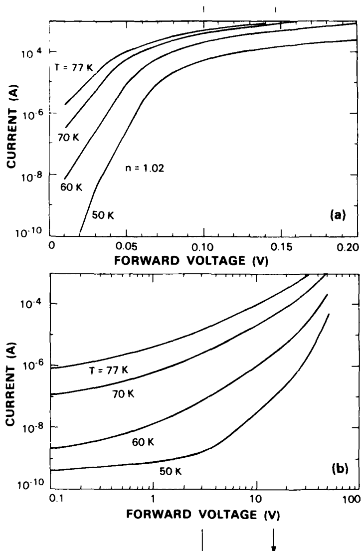
Figure 3-9. (a) Forward and (b) reverse current-voltage characteristics at four temperatures for an IrSi Schottky-barrier detector. The active device area is 1.37 \times 10^{-3} \text{ cm}^2 .
