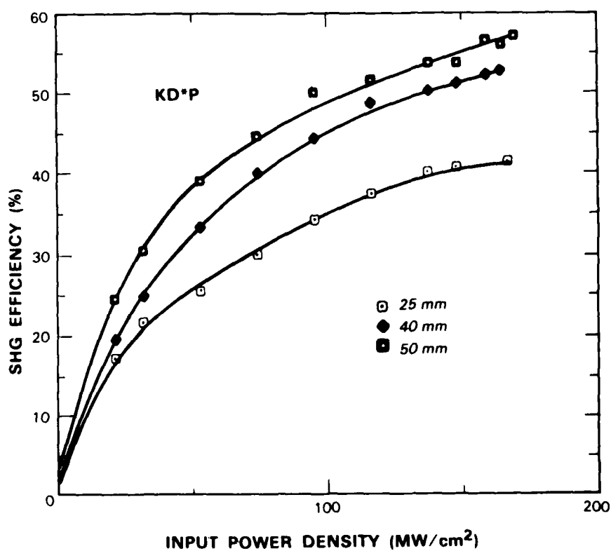
Figure 2-11. Internal frequency-doubling efficiency vs incident power density in KD*P crystals for a macropulse length of 1 \mu s and PRF of 10 Hz.
