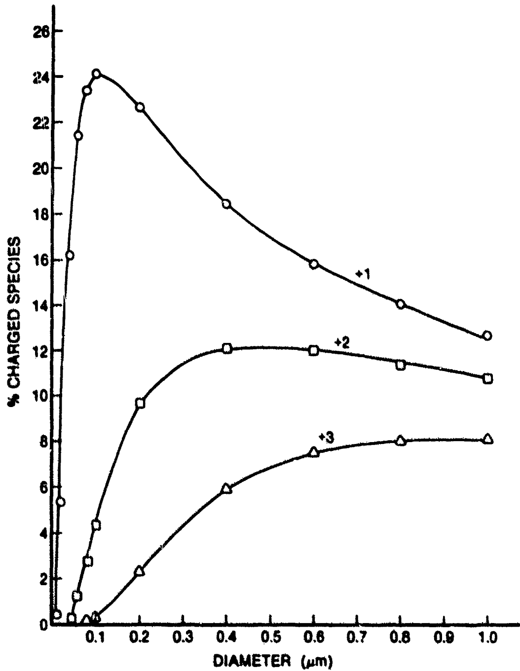
Figure 3: Boltzmann equilibrium distribution of charge in aerosols, as a function of size.
