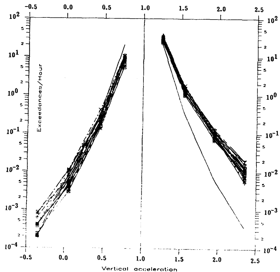
FIG. 5: AIRCRAFT TO AIRCRAFT VARIATION OF LOAD SPECTRA EXPERIENCED BY RAAF CARIBOU AIRCRAFT.
