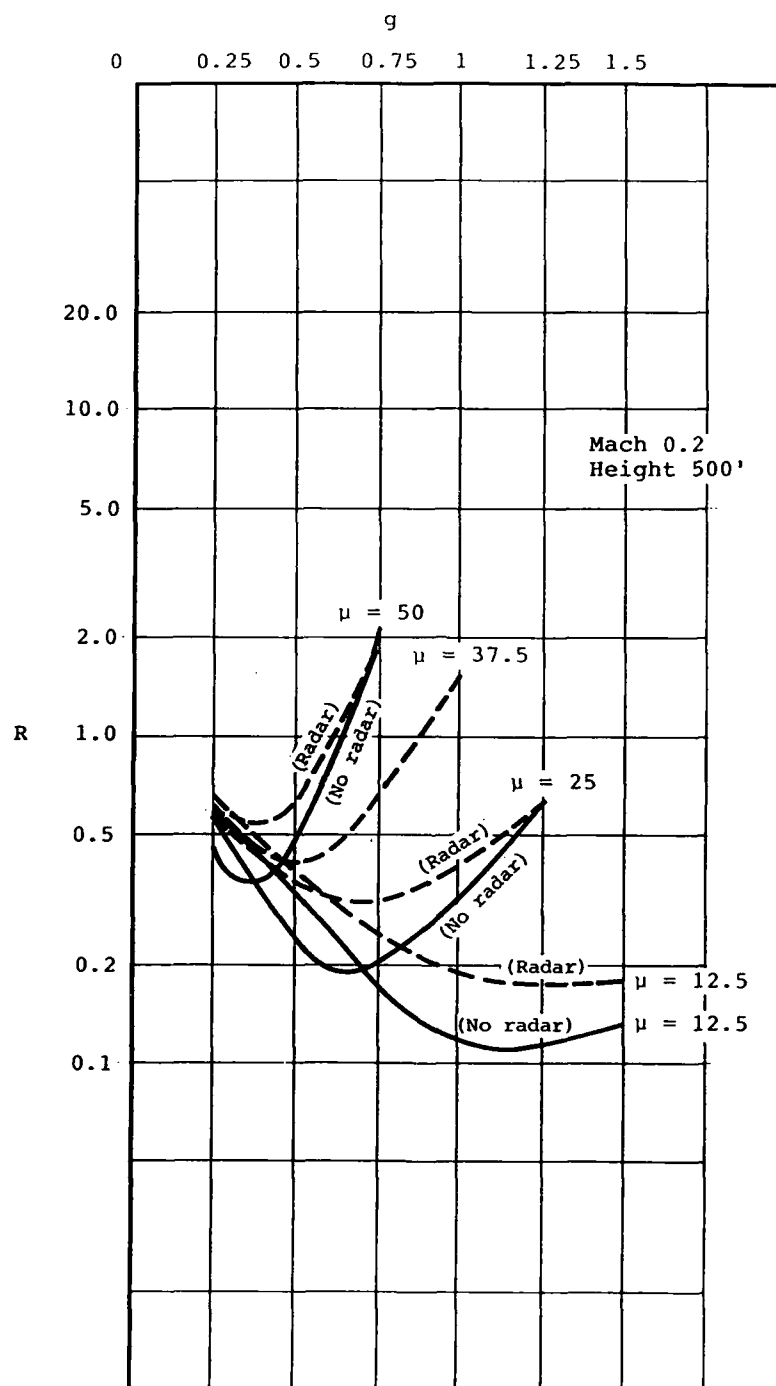
FIG. 12: RATIO, R, OF NUMBER OF LOAD EXCEEDANCES COMPUTED BY POWER SPECTRAL METHOD TO NUMBER COMPUTED BY DISCRETE GUST METHOD FOR AN AIRCRAFT HAVING THE CONFIGURATION OF A CARIBOU AND THE VARIOUS MASS PARAMETERS SHOWN.
