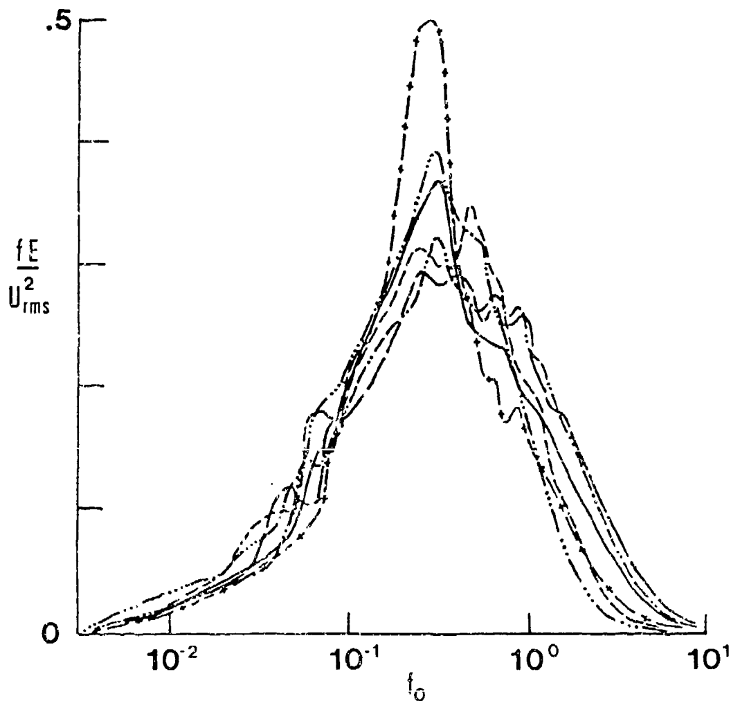
Figure 8. Streamwise Velocity Spectra at Different Distances from the Wall in a Cylindrical Boundary Layer: Re=2000 ; y_+ \approx 2 ; y_+ \approx 13 ; y_+ \approx 37 ; y_+ \approx 78 ; y_+ \approx 158 ; y_+ \approx 399 [Lueptow and Haritonidis. 31 Reprinted with the permission of the American Institute of Physics, copyright 1987.]
